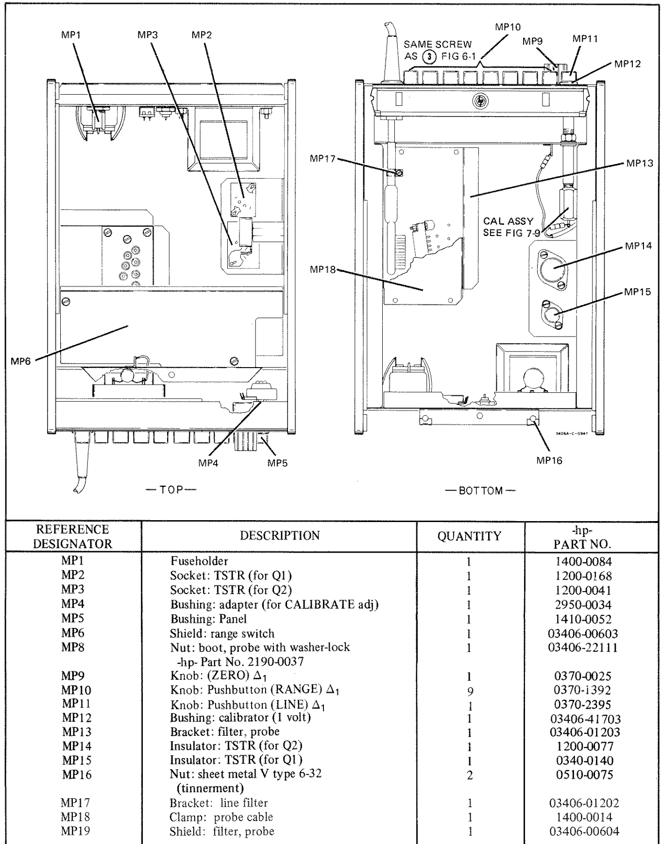
Figure 6-2. Mechanical Parts
