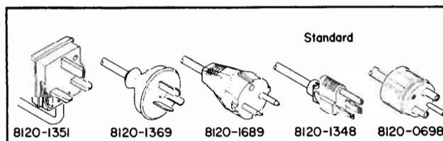
Figure 2-2. Power Cord Receptacles.
