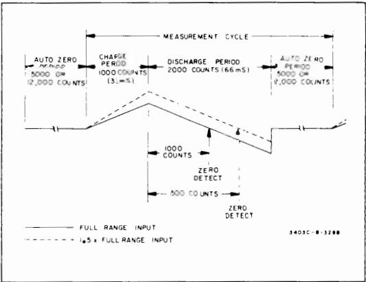
Figure 4-1. Panel Meter Measurement Cycle.
