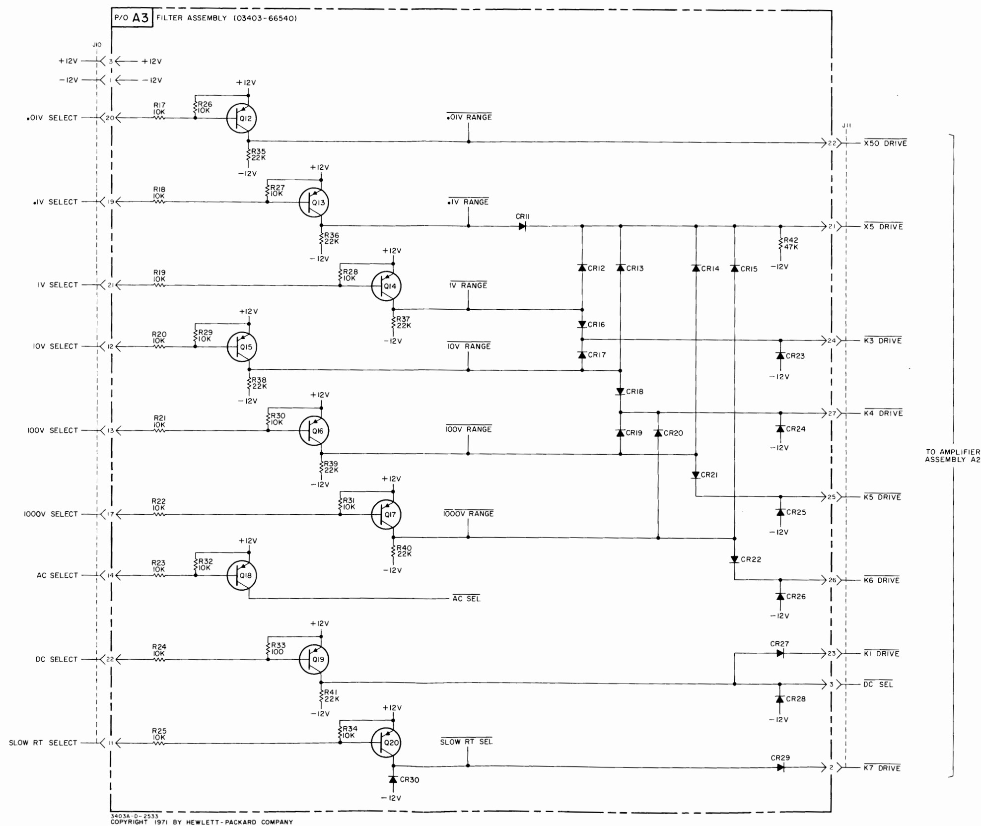
Figure 7-4. Schematic Diagram, AC Converter DC Amp. and Logic Circuits, A3. 7-7/7-8
