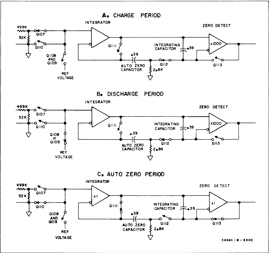
Figure 4-3. Panel Meter Analog Circuits.
