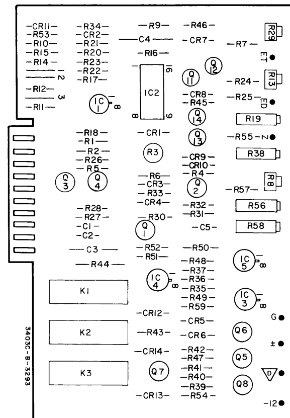
A12 hp Part No. 03403-66592 Rev A
