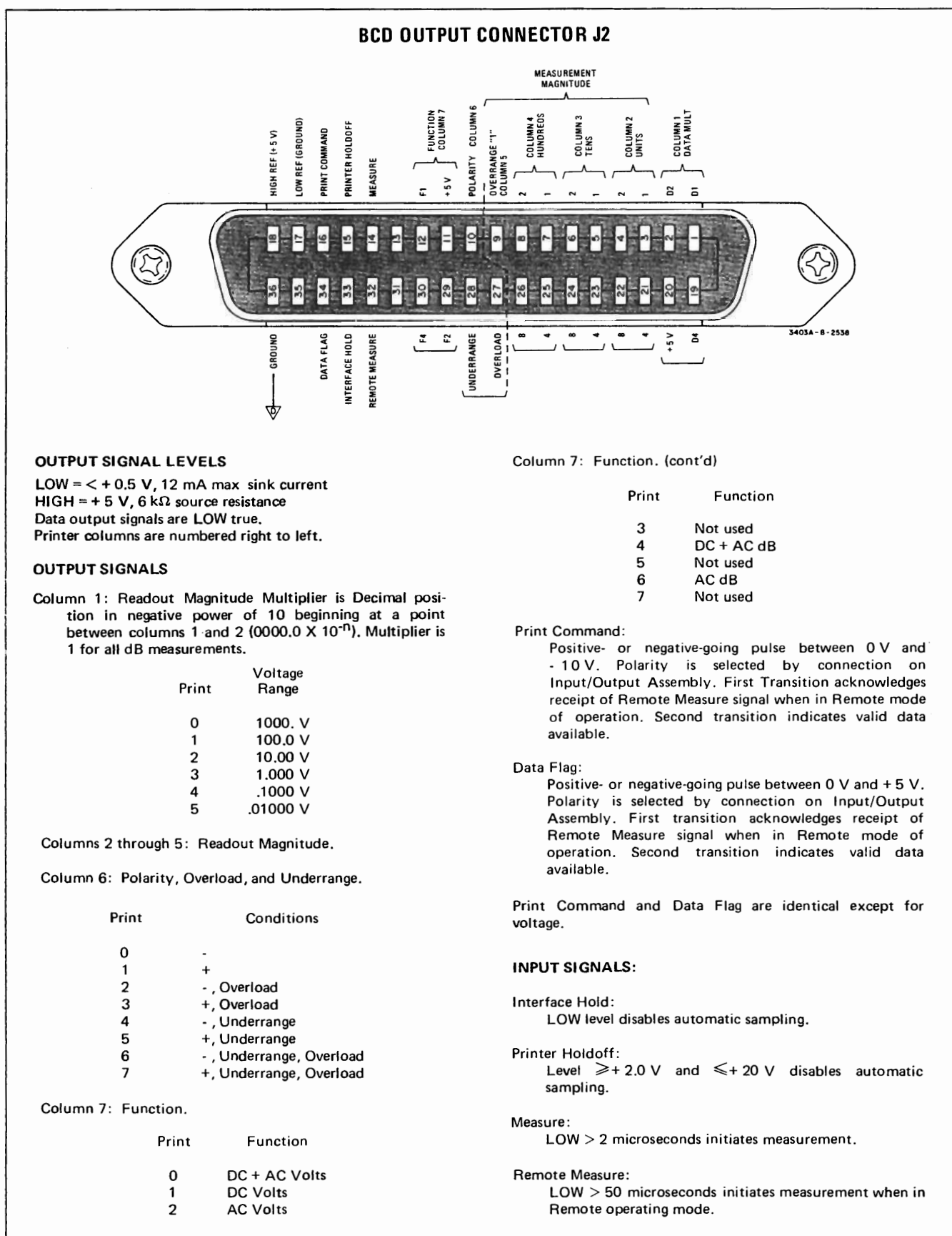
Figure 2-3. BCD Output Connector J2.
