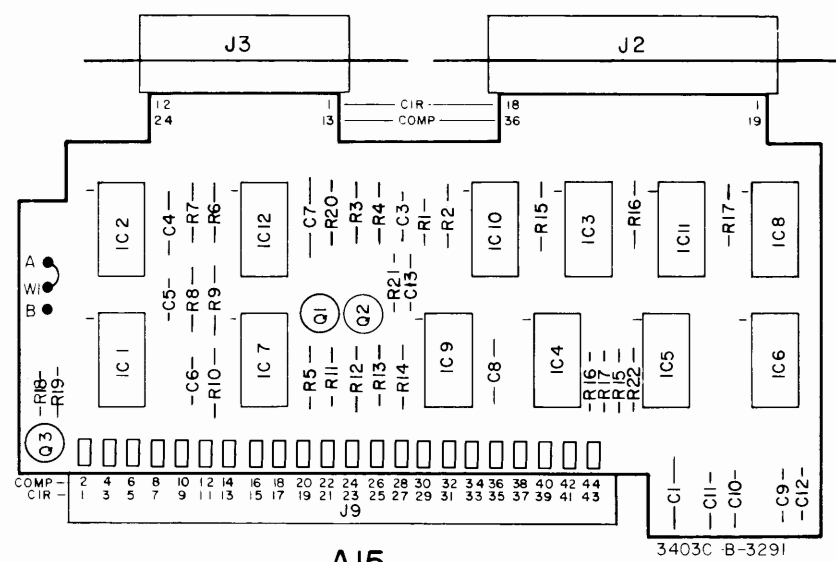
AI5 hp Part No. 03403-66583 Rev. B
