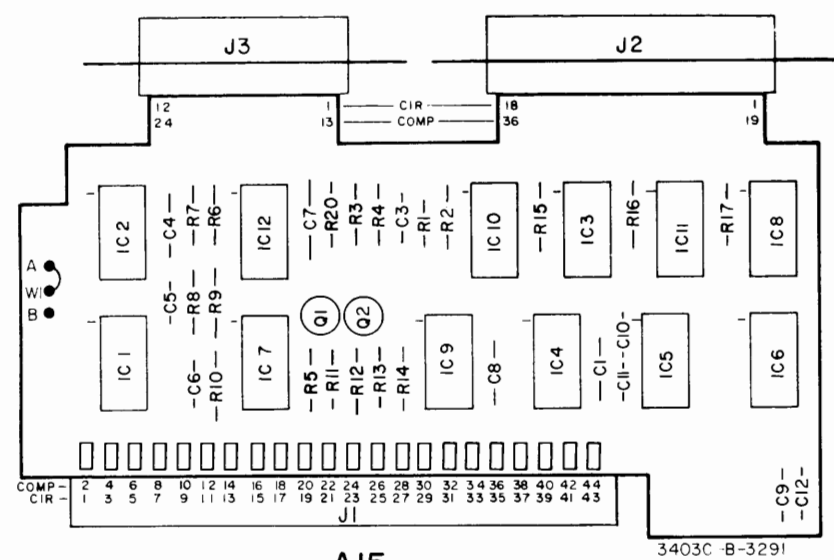
AI5 hp Part No. 03403-66583
