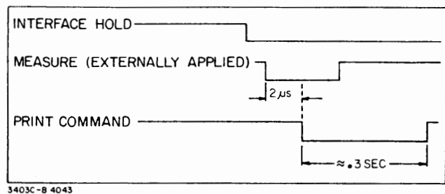
Figure 3-3. Measure Sequence (Non-Remote).
