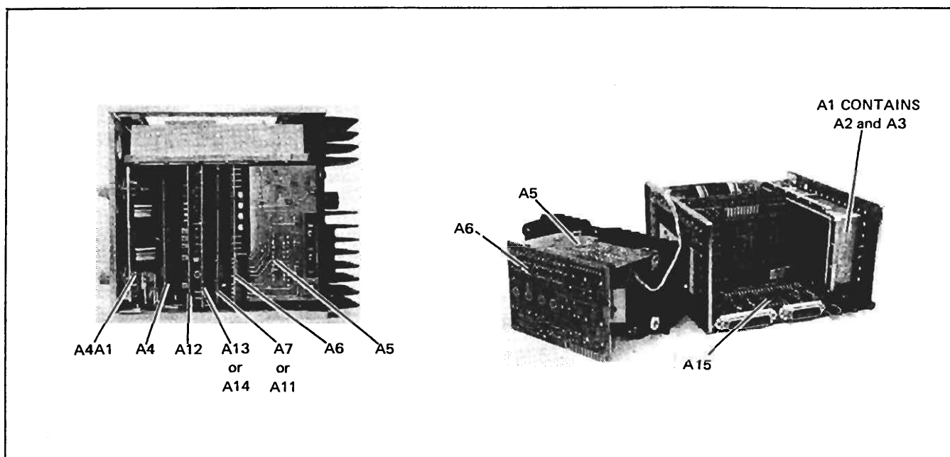
Figure 7-1. Assembly Locations.
