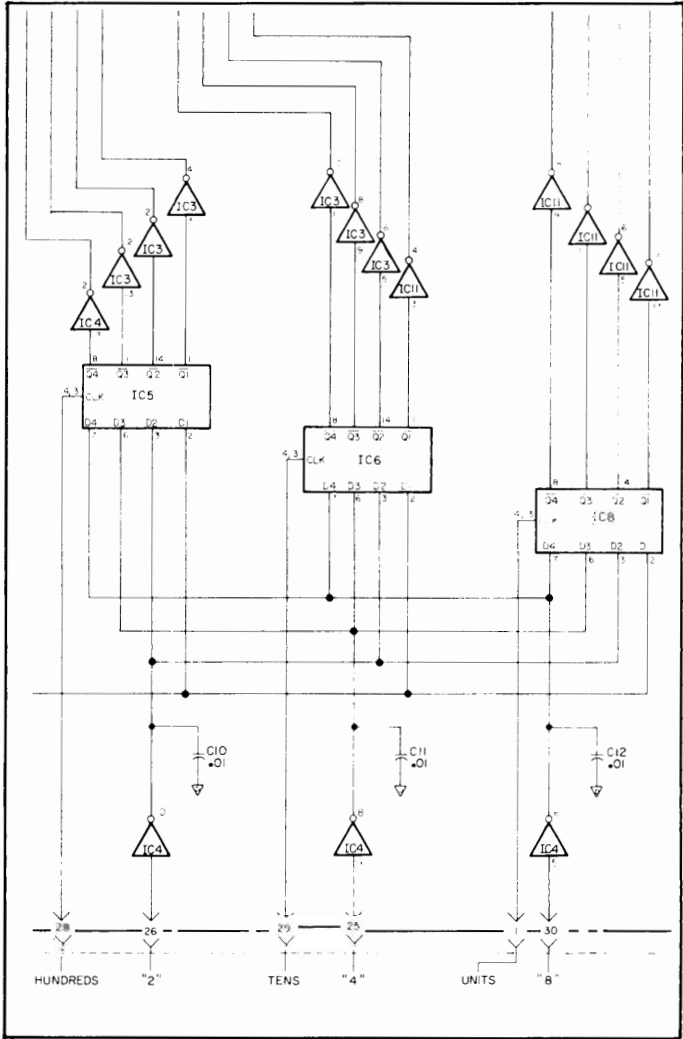
Figure 8-1. p/o A15 Schematic.
