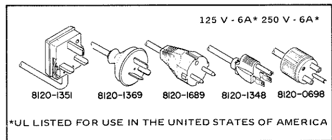
Figure 2-2. Power Cords.
