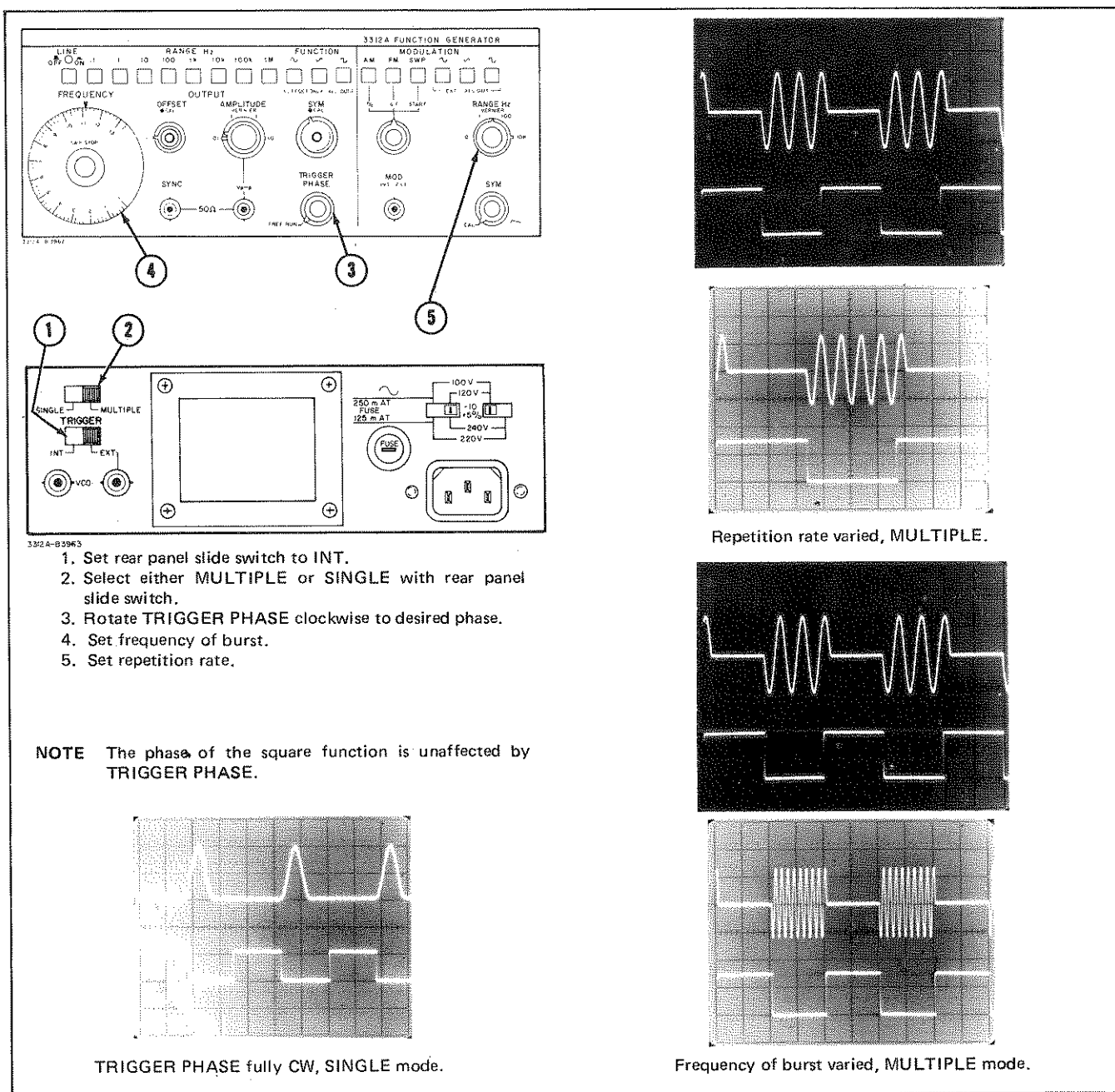
Figure 3-11. Burst Operation.
