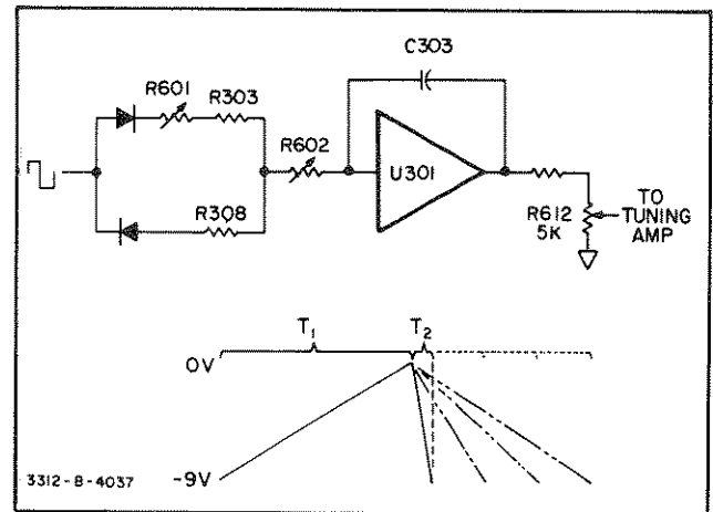
Figure 4-7. Sweep Operation.
