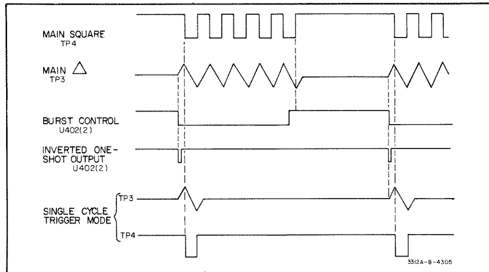
Figure 4-9. Burst Time Relation Waveforms.
