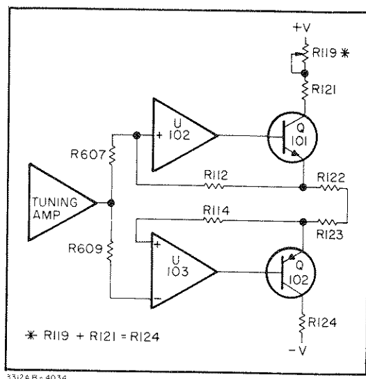
Figure 4-2. Calibrated Symmetry.
