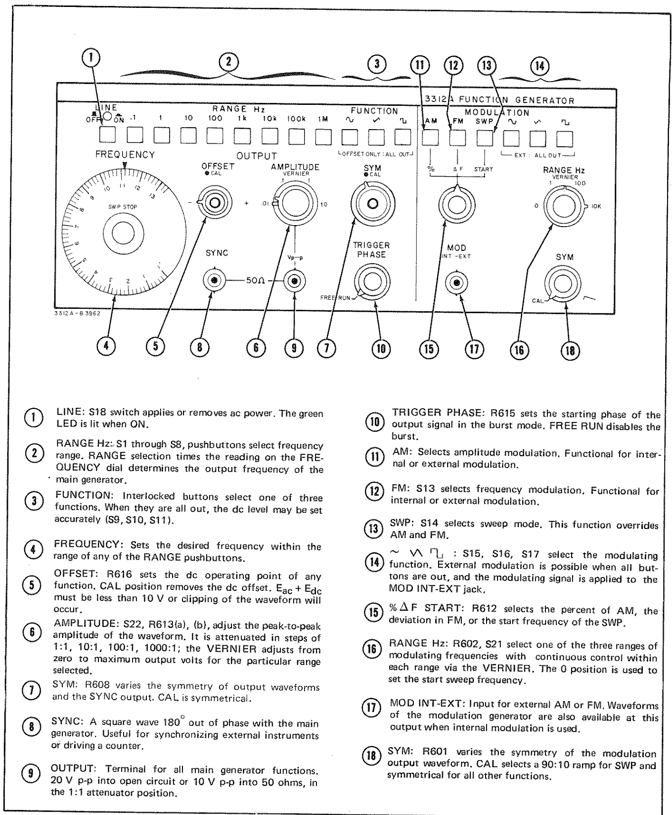
Figure 3-1. Front Panel.
