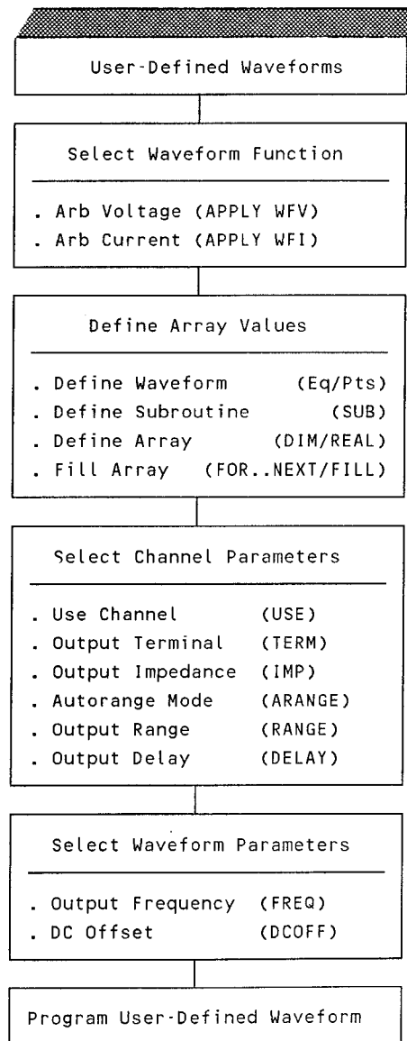
Figure 12-2. User-Defined Waveforms - Selection Steps
