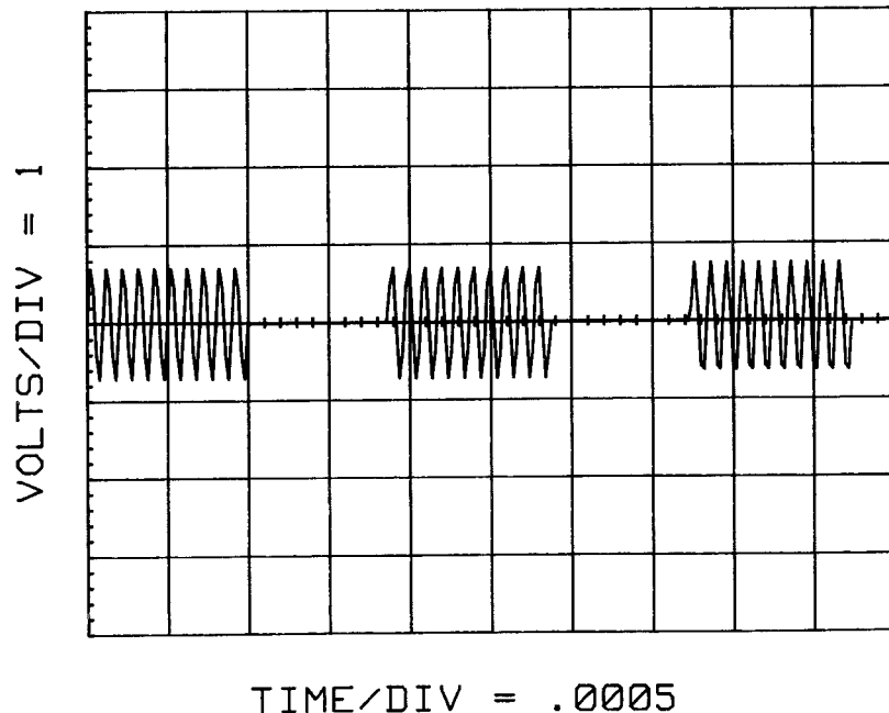
Figure 5-11. Example: Triggered Cosine Waveform
