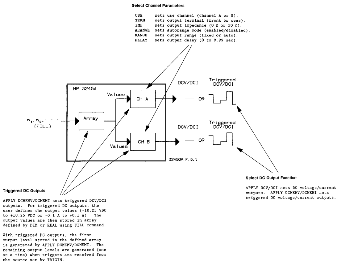
Figure 3-1. DC Outputs - Channel Operation
