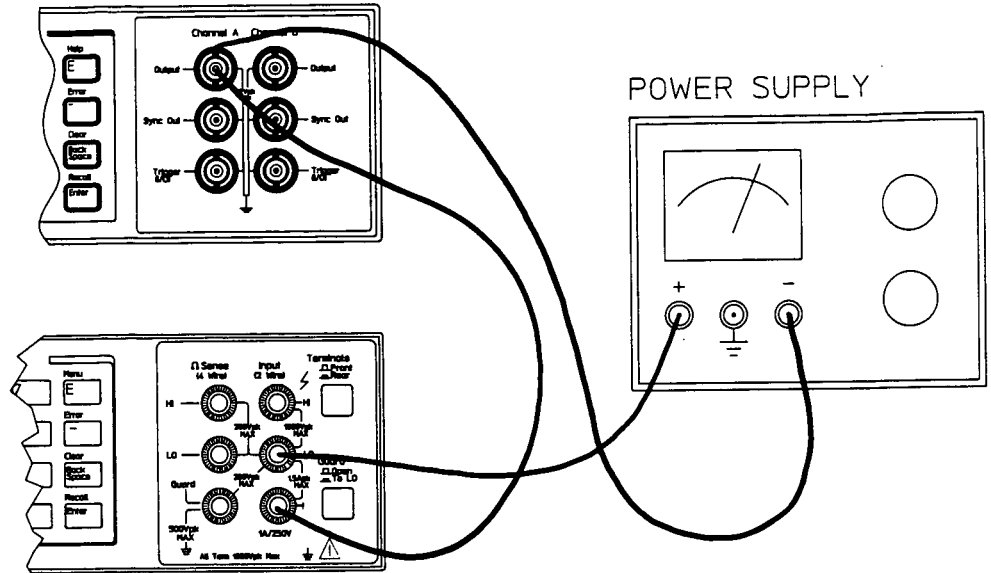
Figure 3-1. DCI Output Resistance and Voltage Compliance Test Set Up
