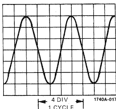
Figure 14. Period Measurement
