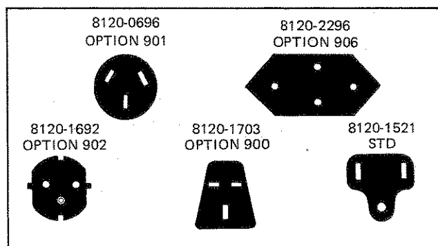
Figure 1. Power Receptacles
