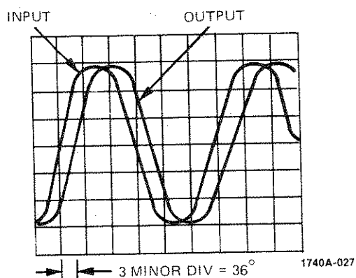
Figure 21. Phase Difference Measurement
