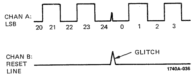
Figure 26. Glitch on Timer Reset Line Causing Timer to Reset Prematurely
