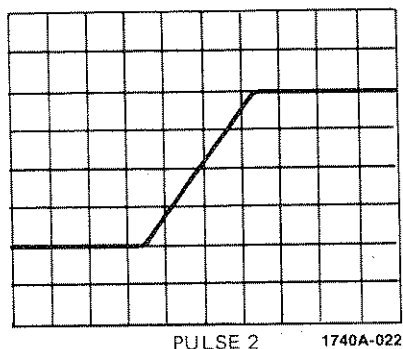
Figure 17c. Time Interval Measurement Using Delayed Time Base - Pulse 2
