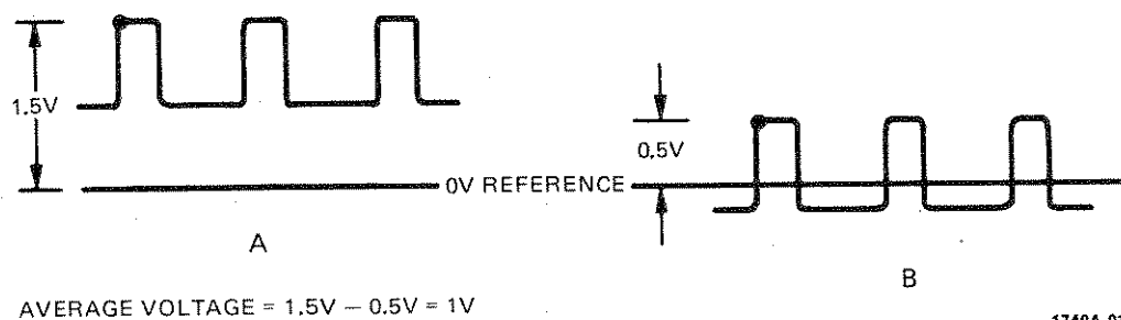
Figure 11. Average Voltage
