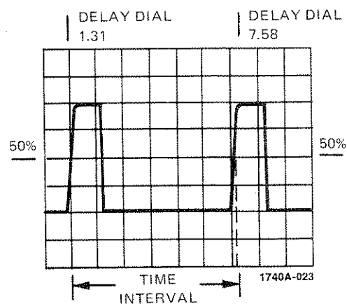
Figure 17d. Time Interval Measurement Using Delayed Time Base - Delay Dial Readings
