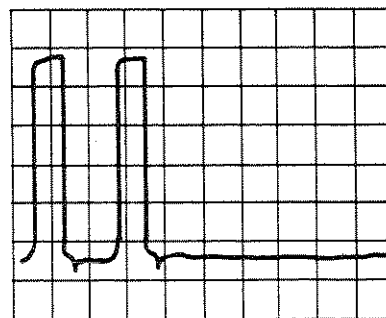
Figure 24b. Multiple Triggering Eliminated With Trigger Holdoff Control
