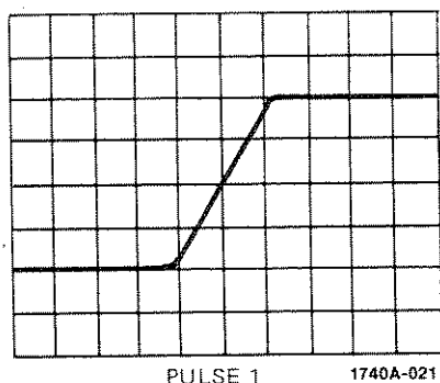
Figure 17b. Time Interval Measurement Using Delayed Time Base - Pulse 1
