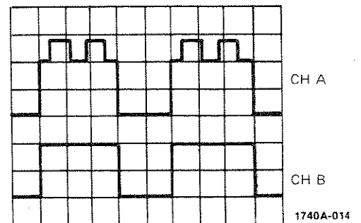
Figure 12a. Channel A With Desired Signal and Unwanted Components. Channel B With Only Unwanted Components.
