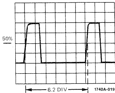
Figure 16. Time Interval Measurement Using Main Time Base
