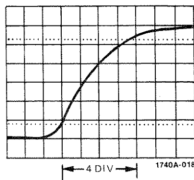
Figure 15. Rise Time Measurement
