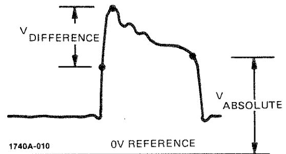
Figure 8. Absolute Voltage and Voltage Difference Measurements
