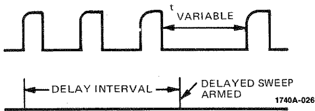
Figure 20. Pulse With Variable Time Duration
