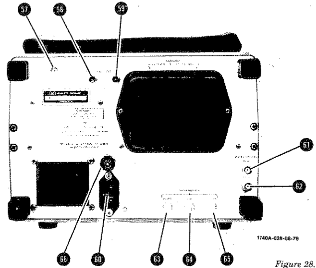
Figure 28. Rear-panel Controls
