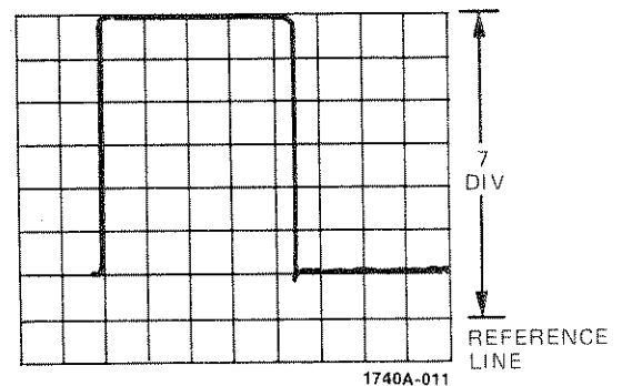
Figure 9. Absolute Voltage Measurement
