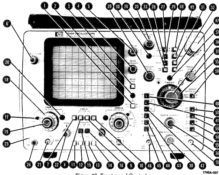
Figure 27. Front-panel Controls
