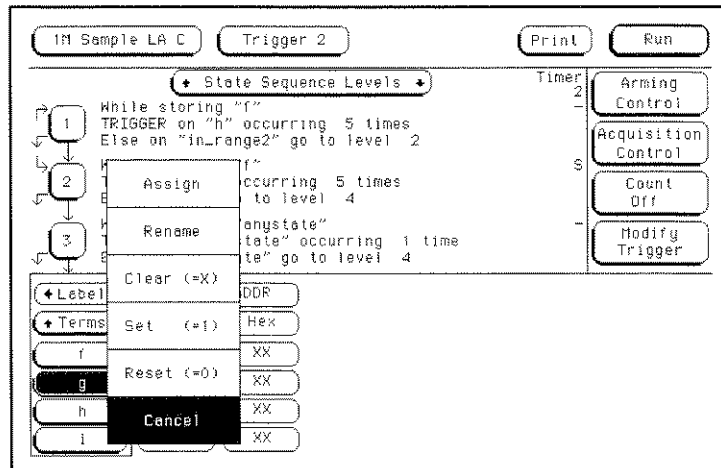
Resource Terms Configuration Menu
