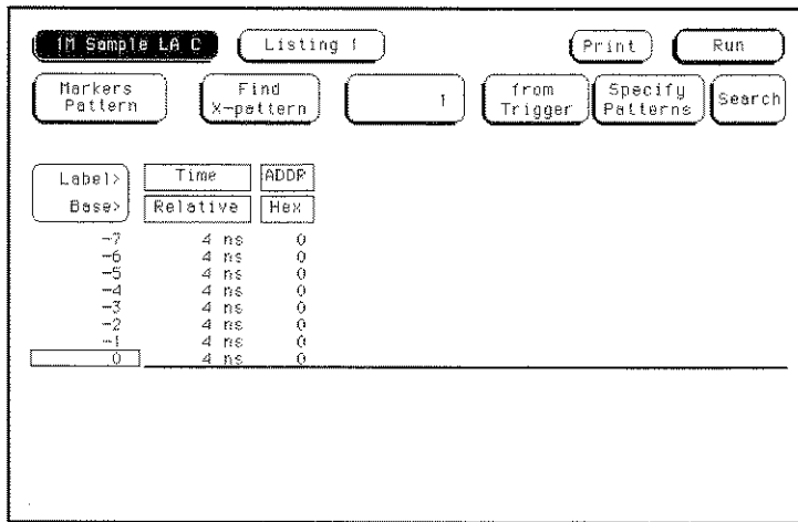
Find X-pattern / O-pattern Field
