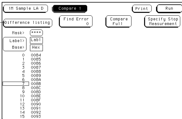
Difference Listing Field
