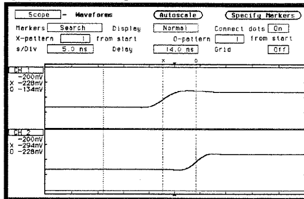
Figure 25-26. Waveform Display
