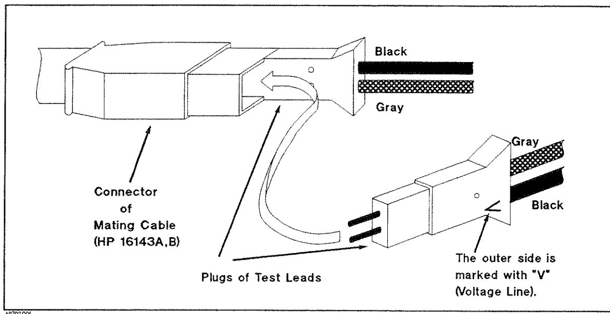
Figure 2-4. Connecting Test leads to HP 16143A, B
