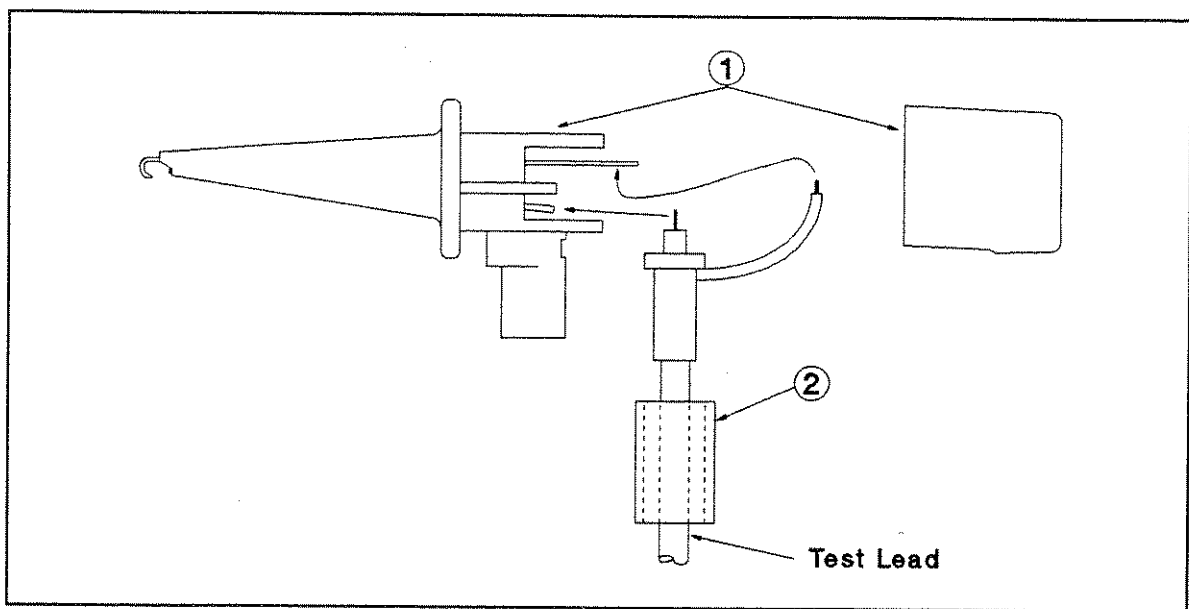
Figure 4-1. Kelvin Clip Connections
