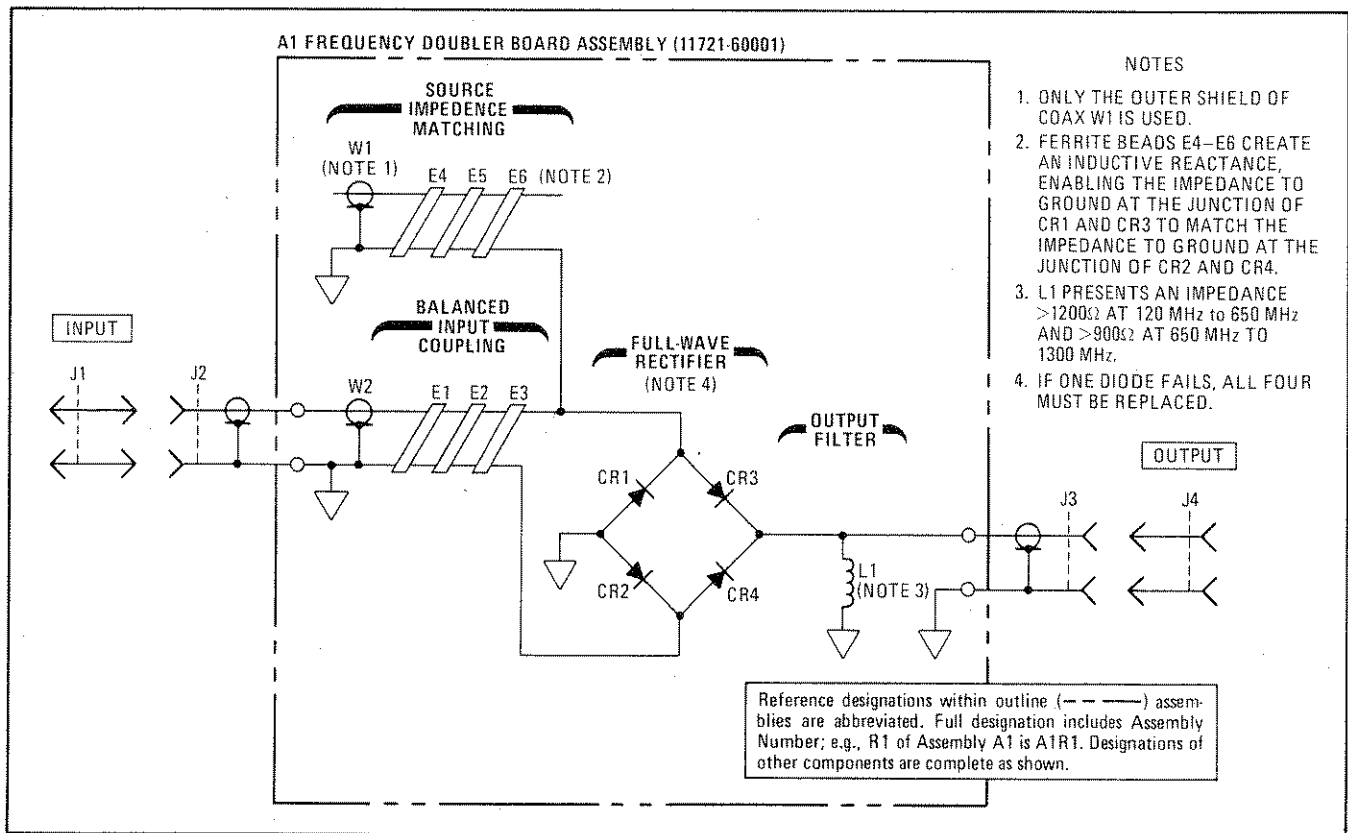
Figure 4. Schematic Diagram
