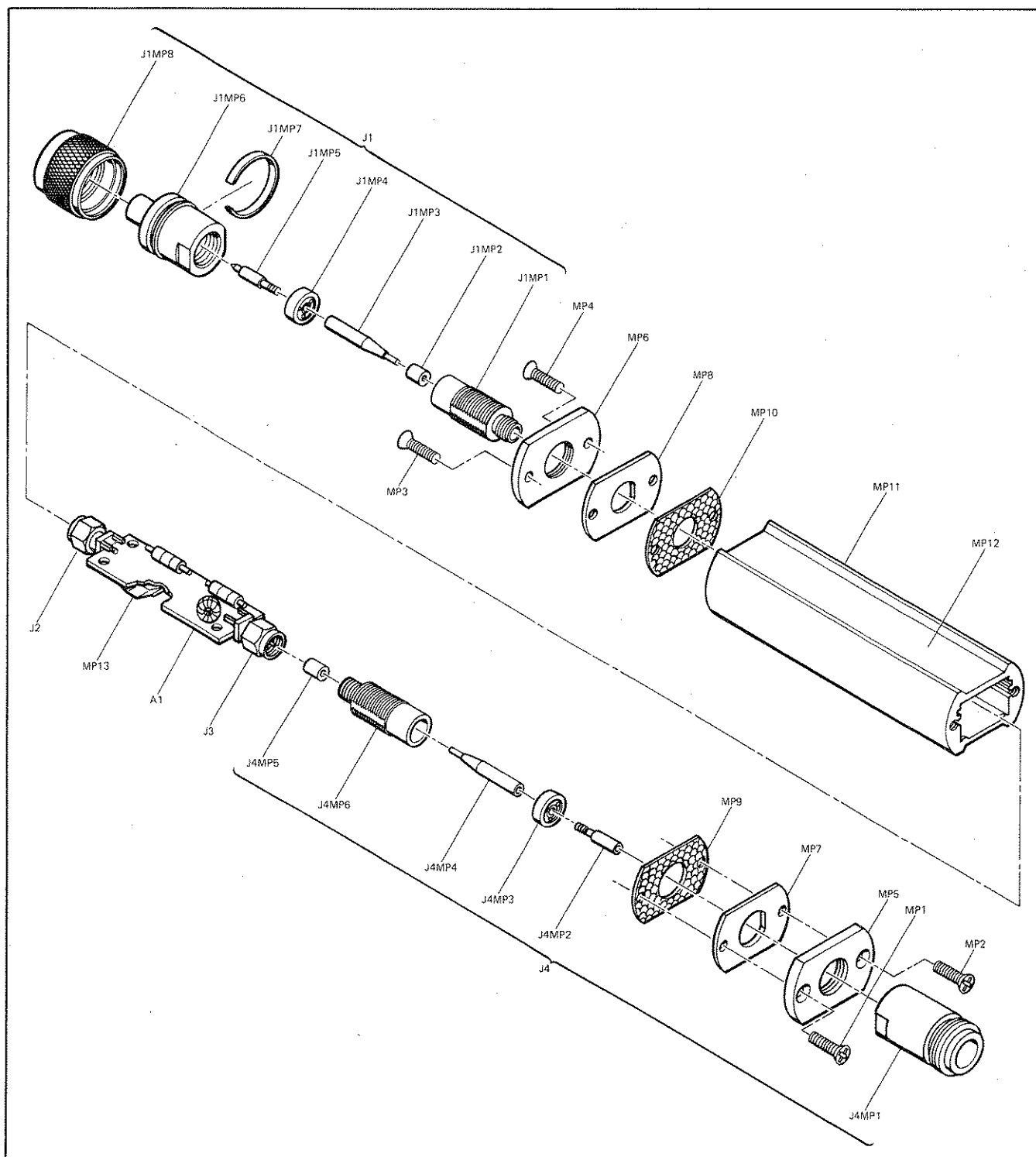
Figure 2. Illustrated Parts Breakdown
