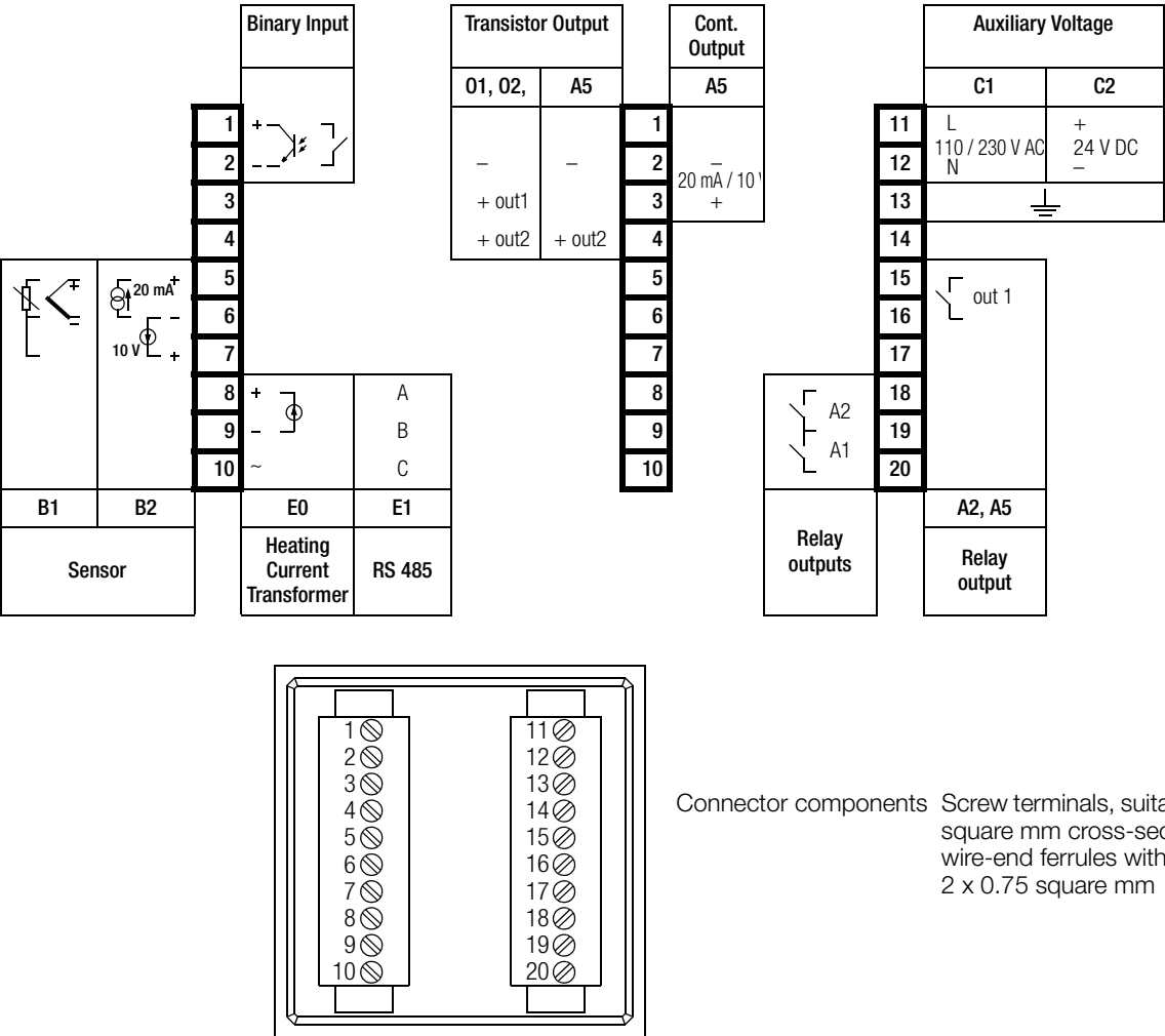
Figure 5: Connector Terminal Positions
