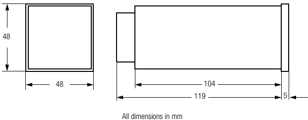
Figure 4: Housing Dimensions
