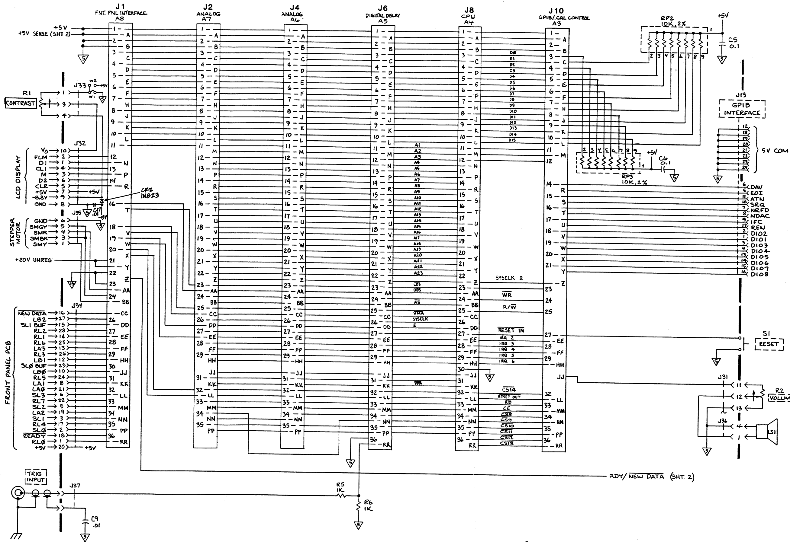
Interconnect Circuit Schematic (A1) DWG# 21088 Rev A Sheet 1 of 3 8-6
