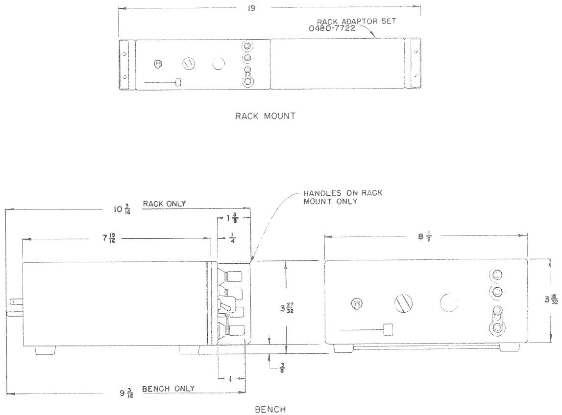
Figure 2-1. Dimensions of the generator, in inches.
