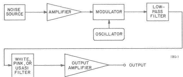
Figure 4-1. Block diagram of the 1382 Random-Noise Generator.
