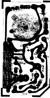
Figure 10. Etched Board Layout of the Type 1232-A Tuned Amplifier and Null Detector.
