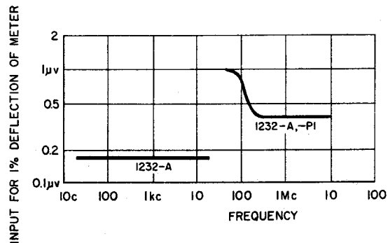
Sensitivity and frequency range of Type 1232-A.
