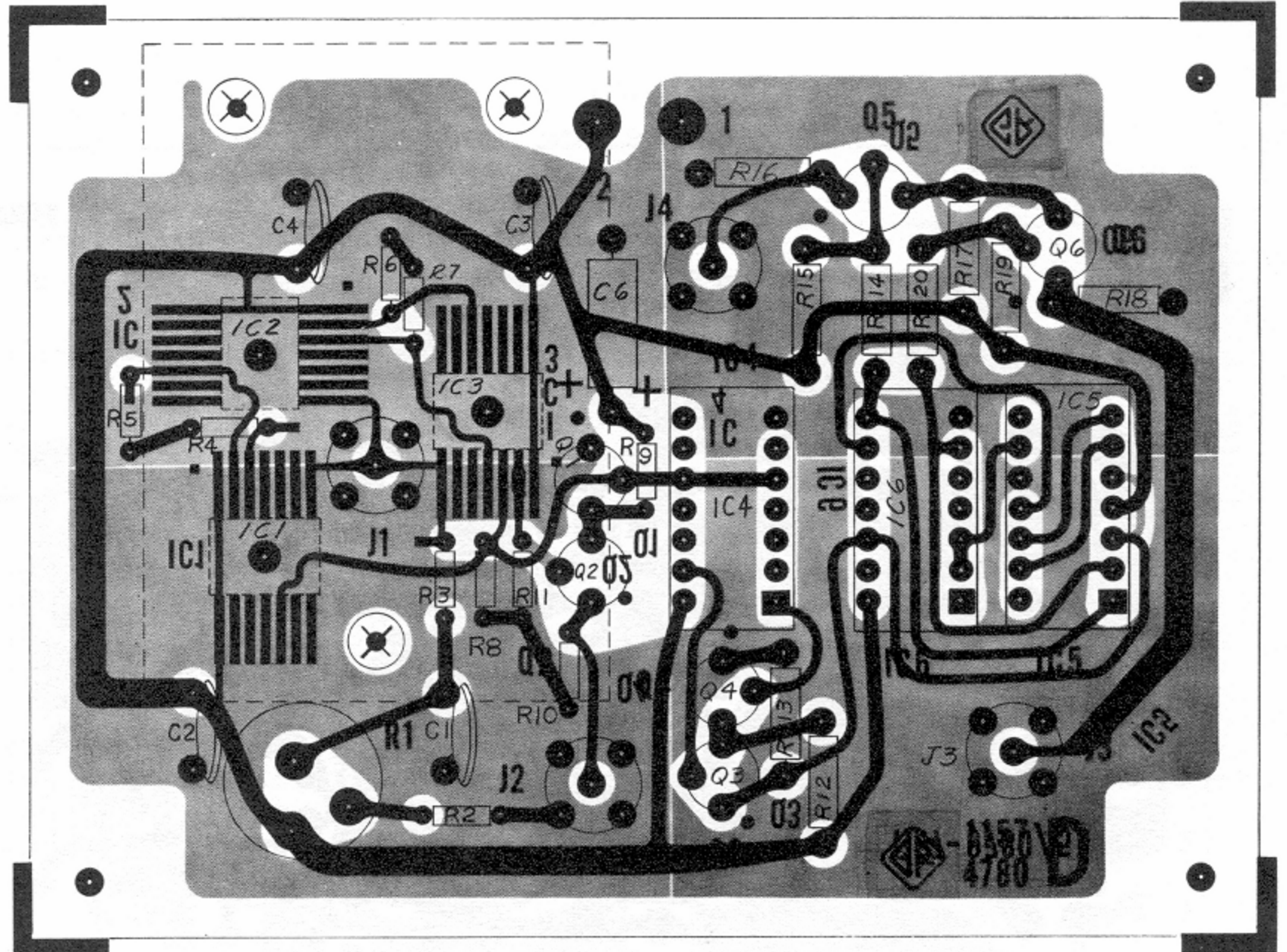
Figure 6-8. D-assembly etched-circuit board (P/N 1157-4780).
