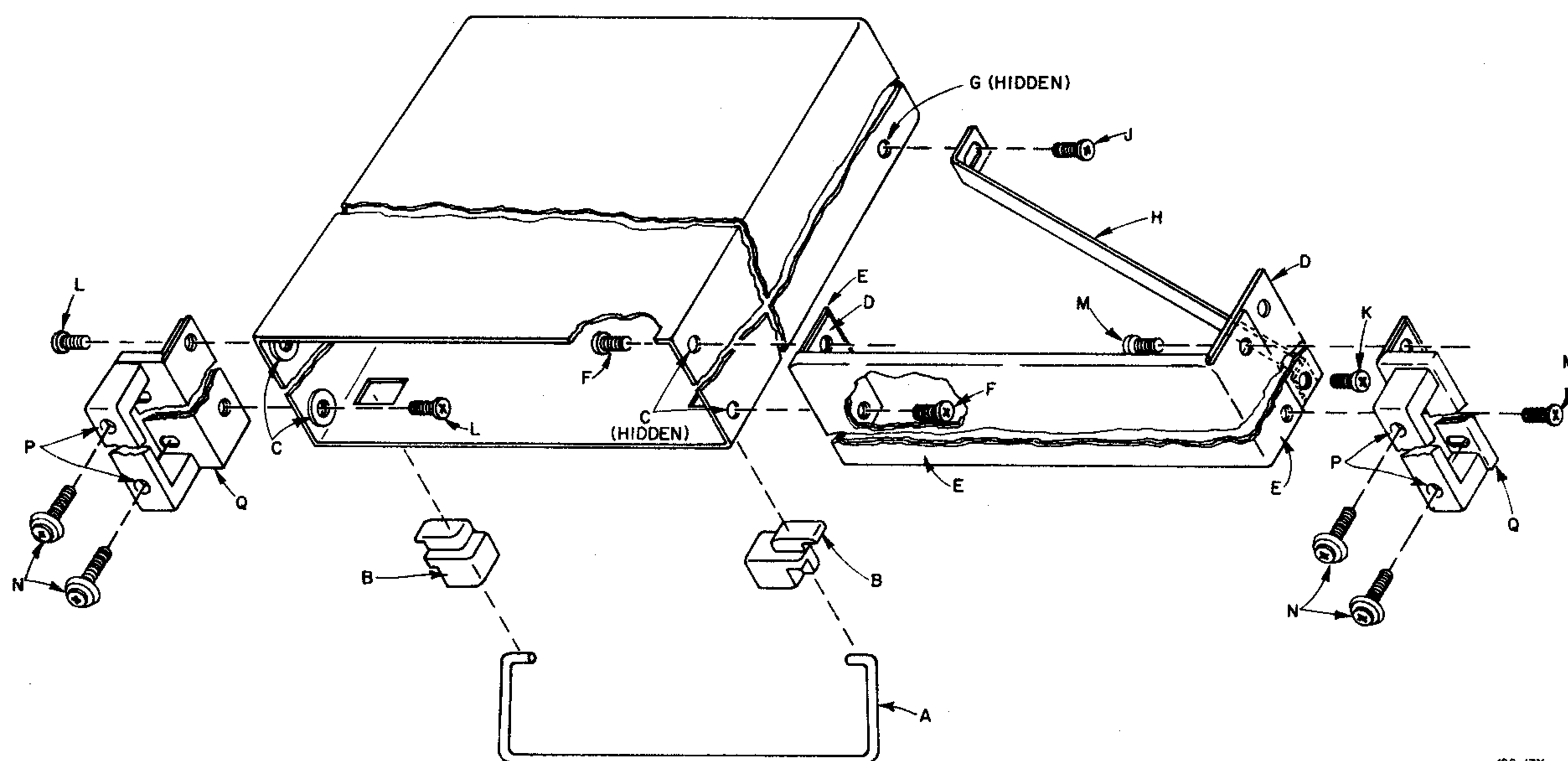
Figure 2-2. Method of mounting scaler in a relay rack.
