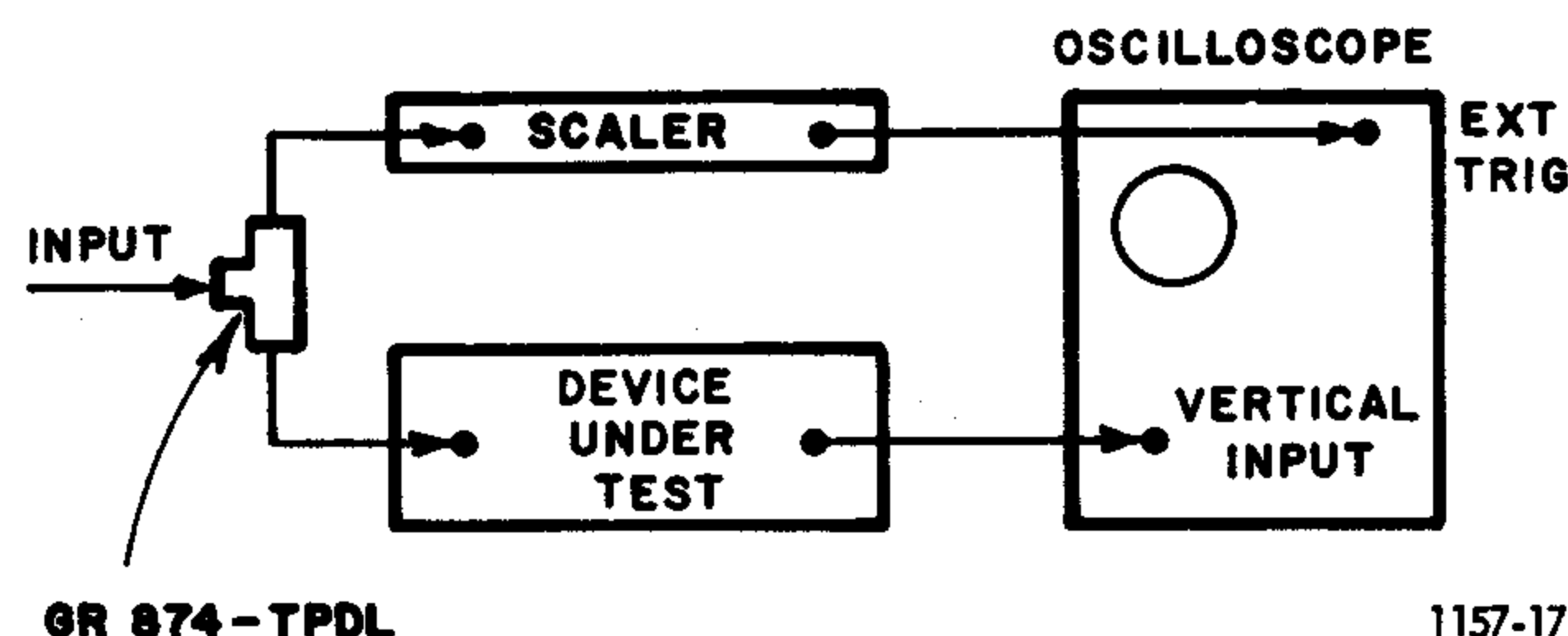
Figure 3-2. Use of scaler to trigger a scope.
