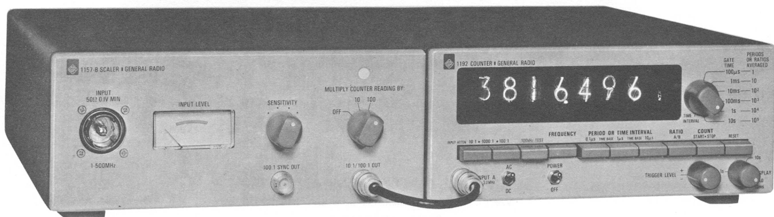
Scaler/Counter Combination — GR 1192-Z.
