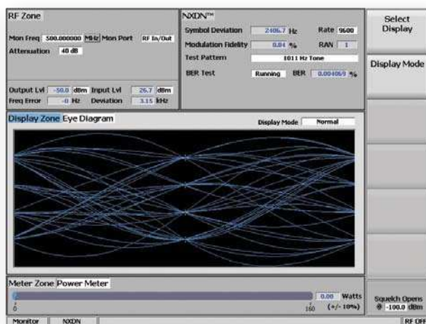
NXDN Test Suite: Signal Quality Metrics and Eye Diagram
