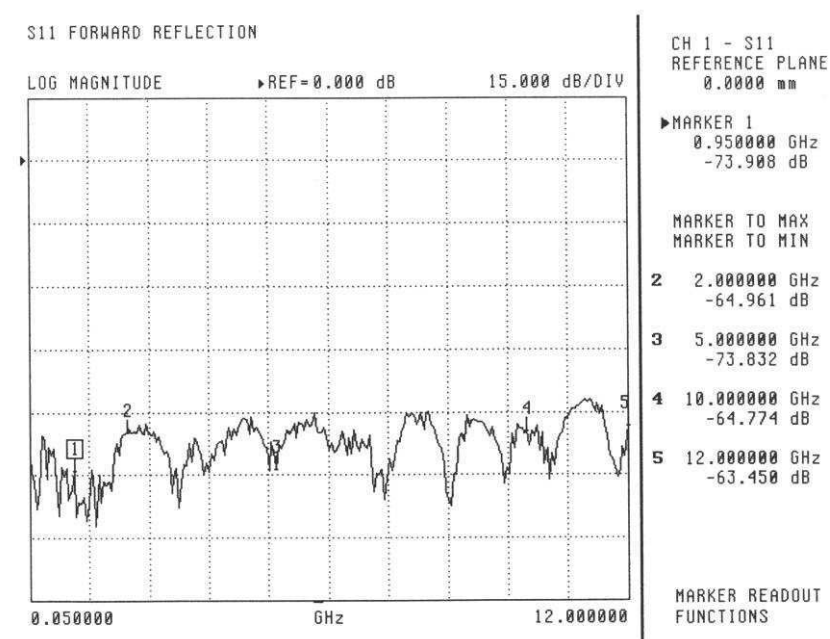
Figure 16: GPC-N test: Thru Line Return Loss
