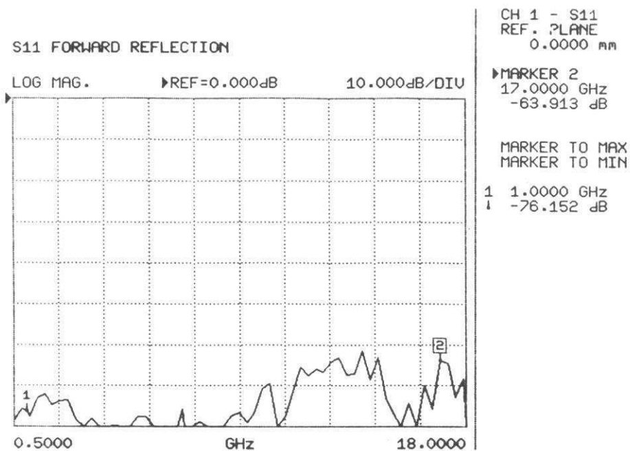
Figure 17: GPC-7 test: Thru Line Return Loss
