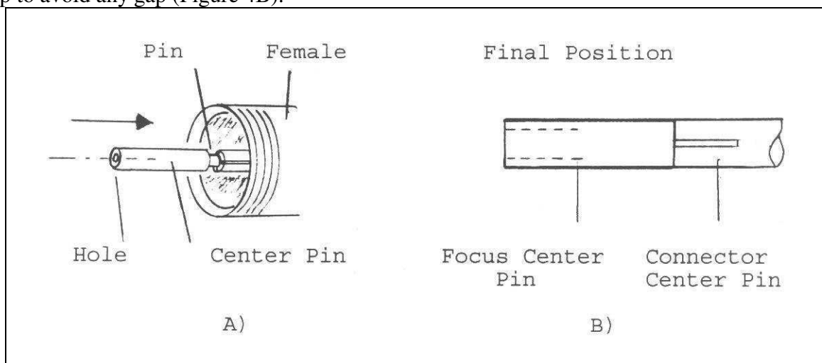
Figure 4: Delay Line inside the female connector for 1.85, 2.4, 2.9 & 3.5mm
