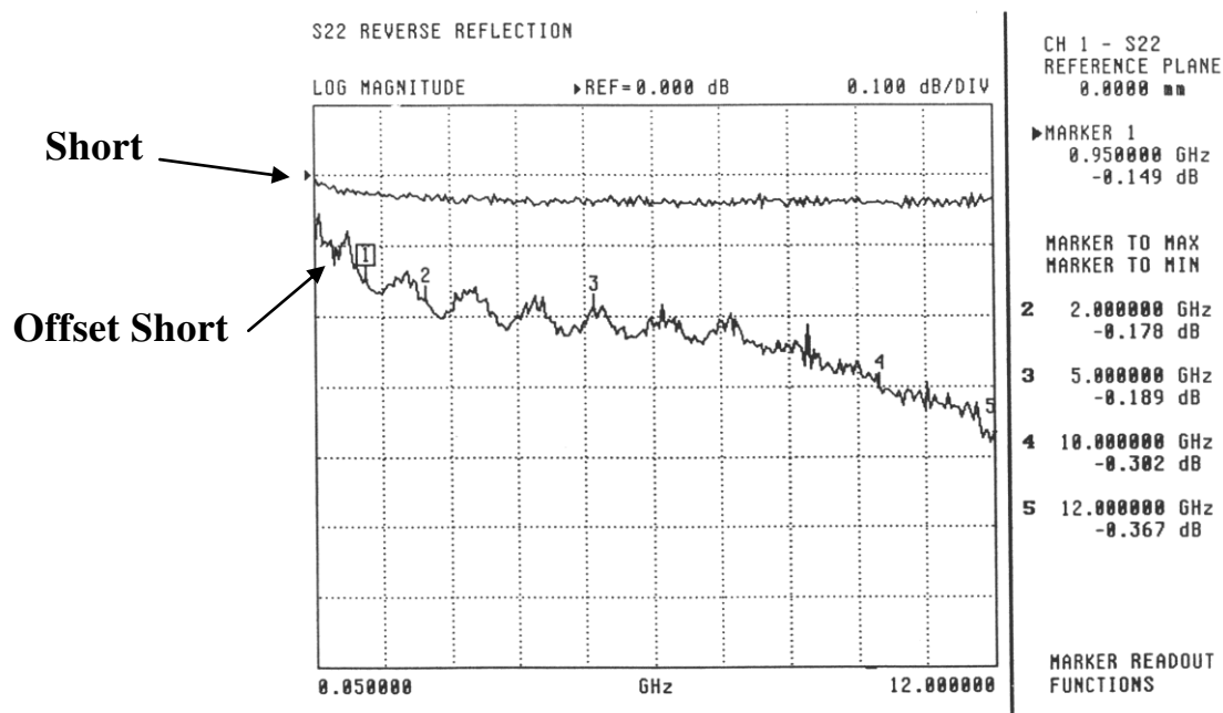
Figure 8: GPC-N test: 1-Direct Short, 2- Offset Short (10 cm)
