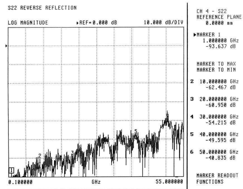
Figure 20: GPC-2.4 test: Thru Line Return Loss
