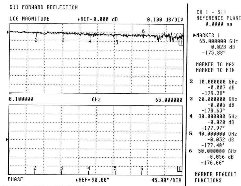
Figure 13: GPC-1.85 test: Short
