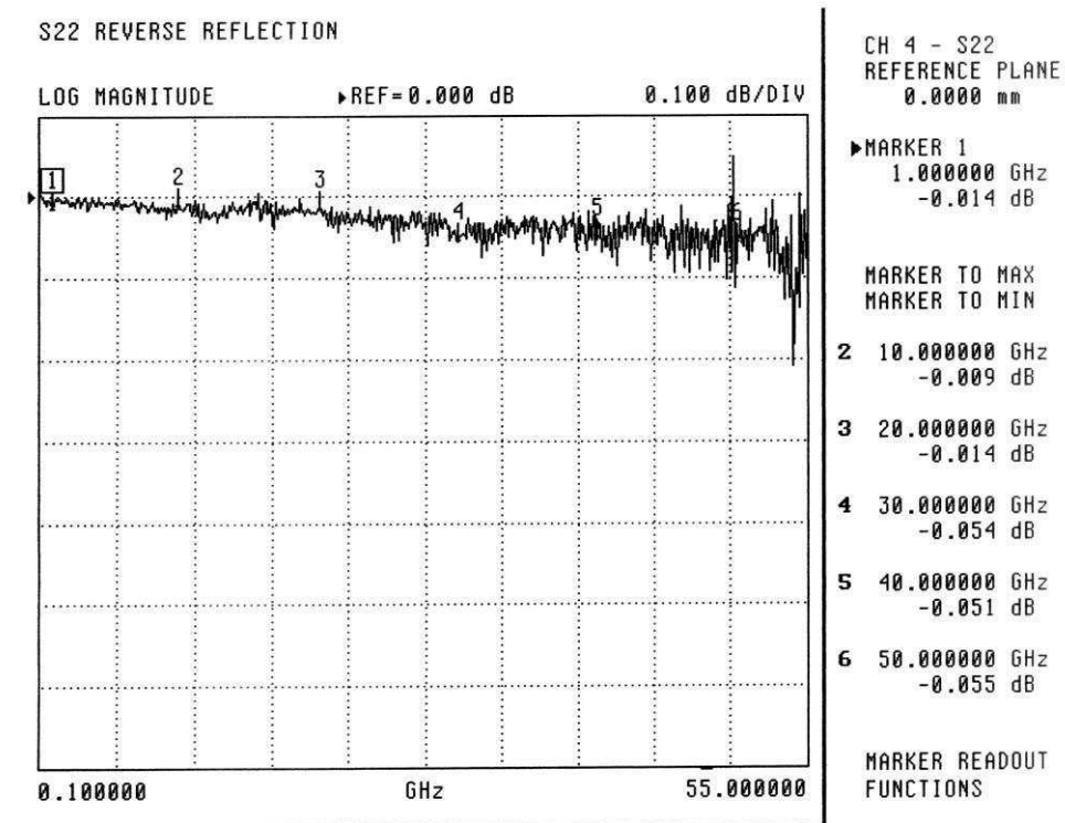
Figure 12: GPC-2.4 test: Direct Short
