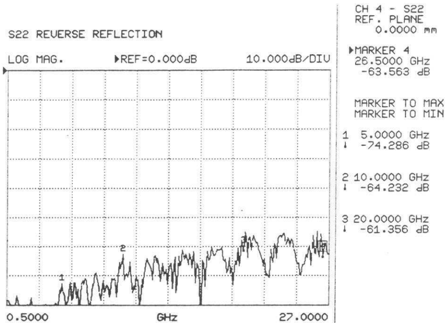
Figure 18: GPC-3.5 test: Thru Line Return Loss
