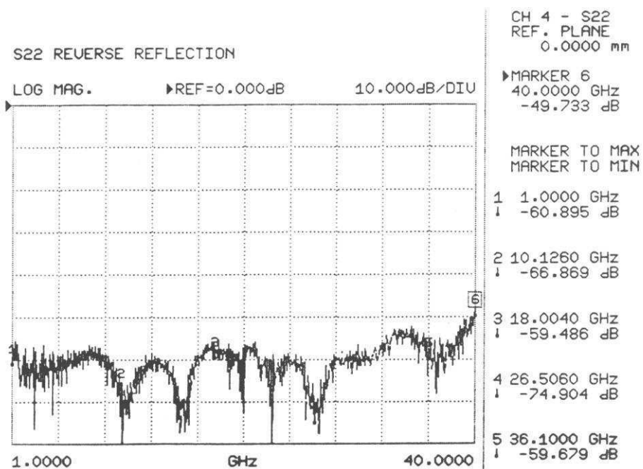
Figure 19: GPC-2.92 test: Thru Line Return Loss
