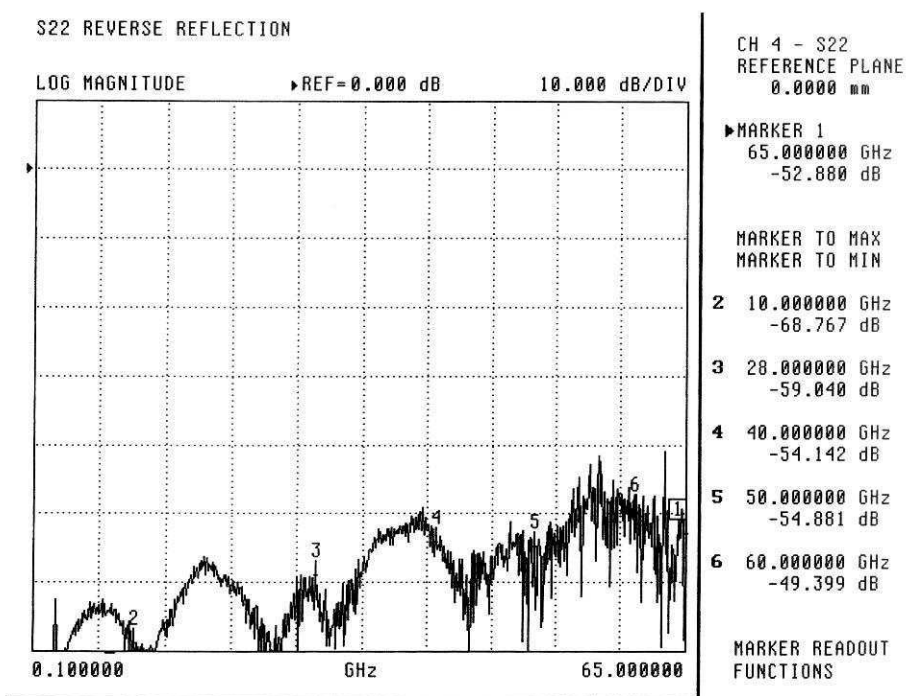
Figure 22: GPC-1.85 test: Thru Line Return Loss
