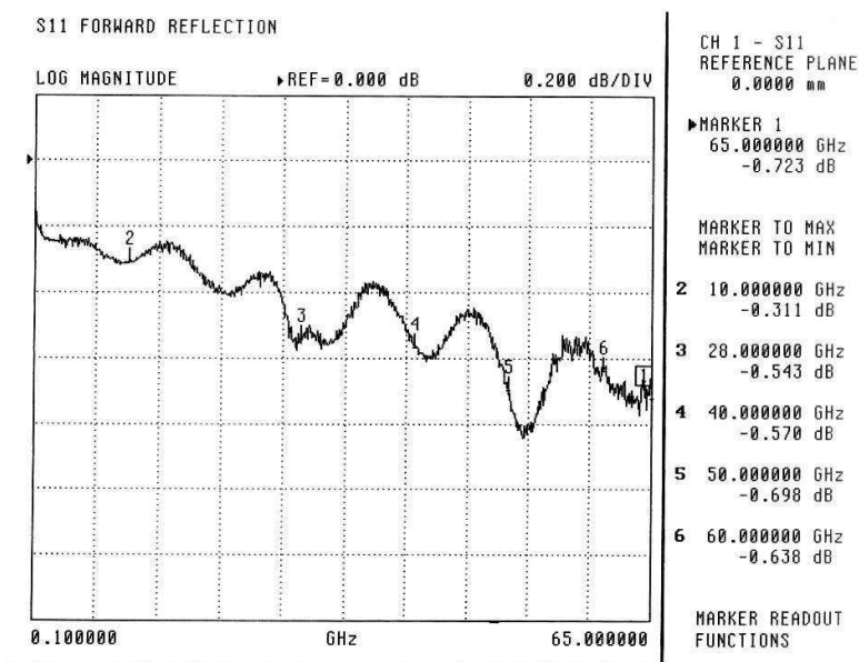
Figure 14: GPC-1.85 test: Offset Short
