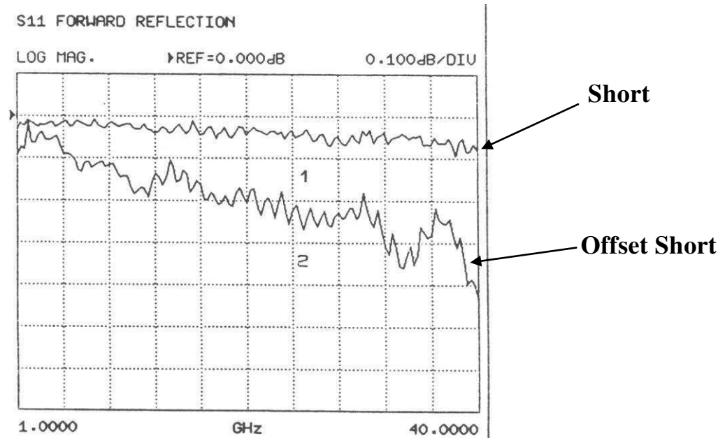
Figure 11: GPC-2.92 test: 1-Direct Short, 2- Offset Short (1.6 cm)
