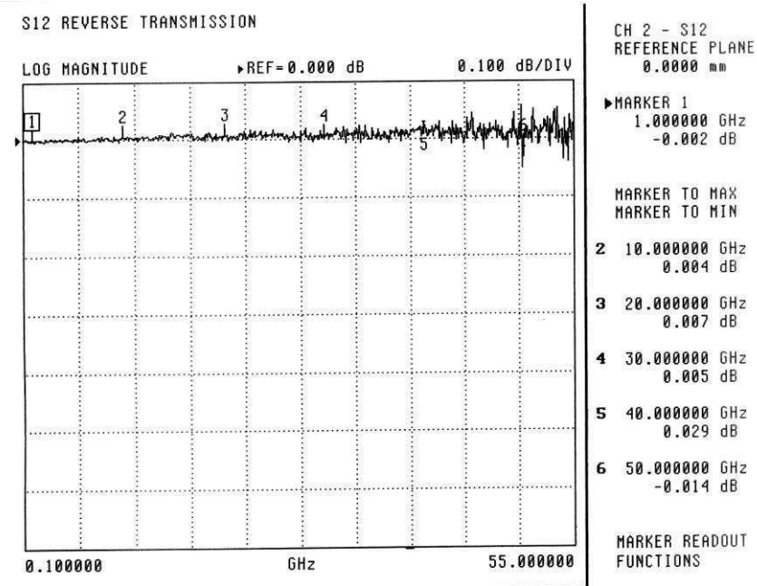
Figure 21: GPC-2.4 test: Thru Line Reverse Transmission
