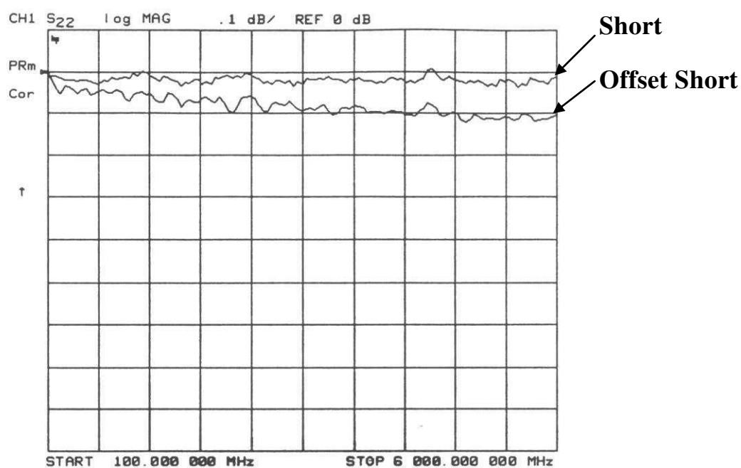
Figure 7: GPC-7/16 test: 1-Direct Short, 2- Offset Short (40 cm)
