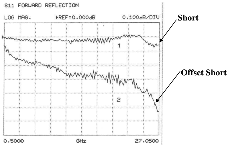
Figure 10: GPC-3.5 test: 1-Direct Short, 2- Offset Short (4.3 cm)
