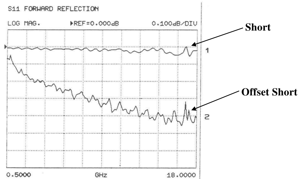
Figure 9: GPC-7 test: 1-Direct Short, 2- Offset Short (10 cm)
