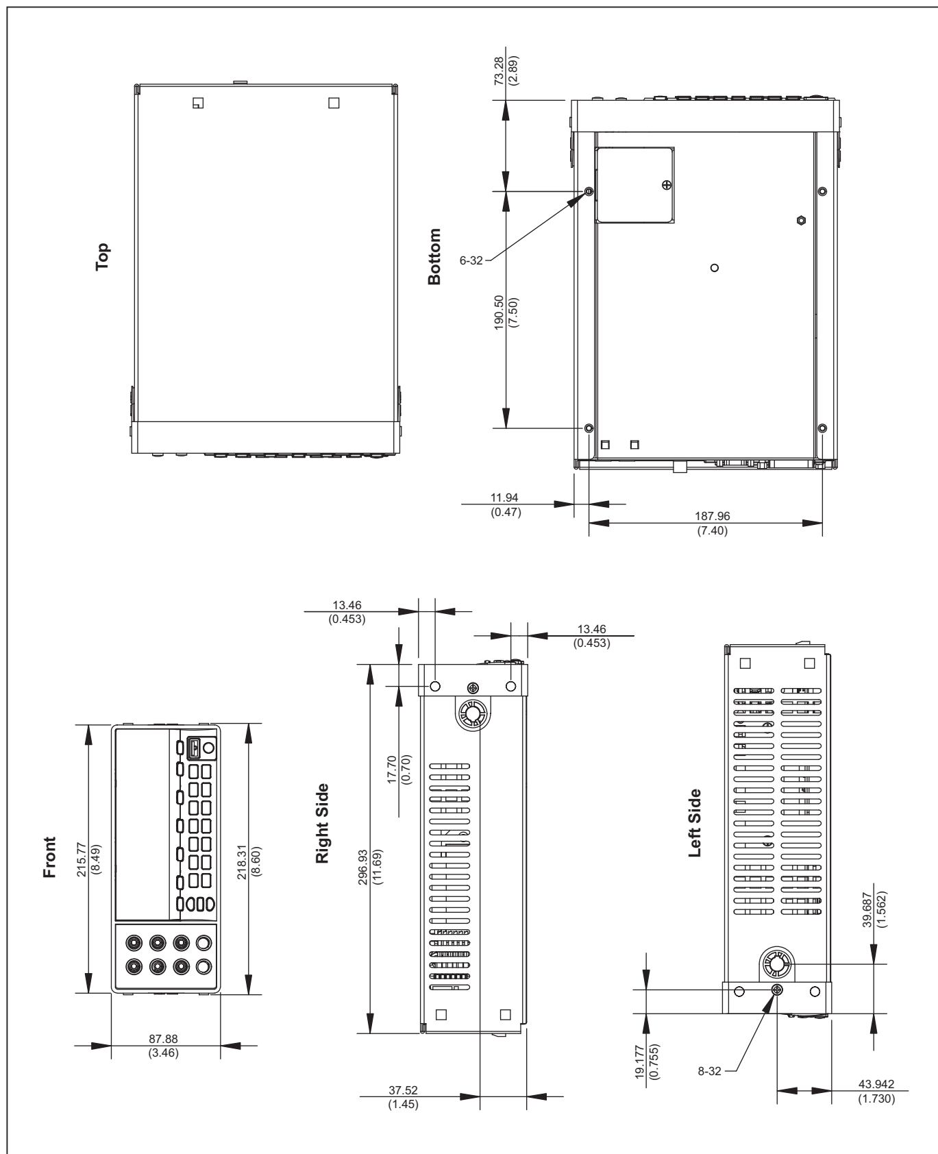
Figure 4. Dimensions
