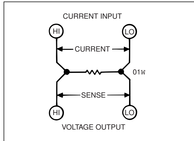
Figure 2. Current Shunt
