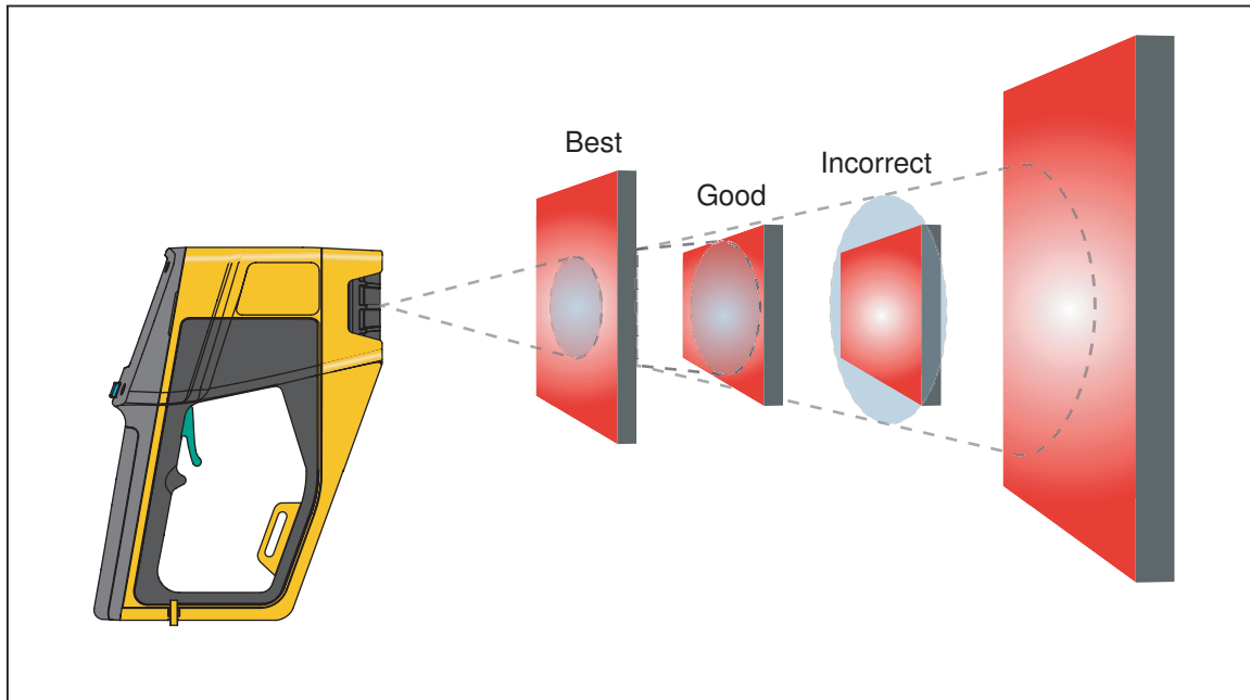
Figure 2-4. Correct Field of View
