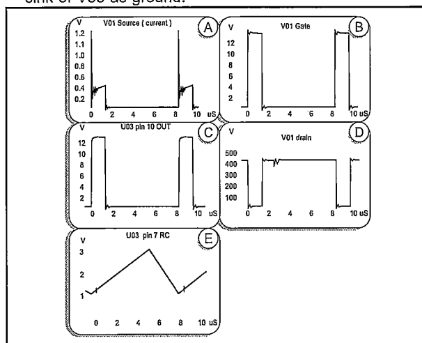
Figure 5-8 Typical curves of the power supply.
