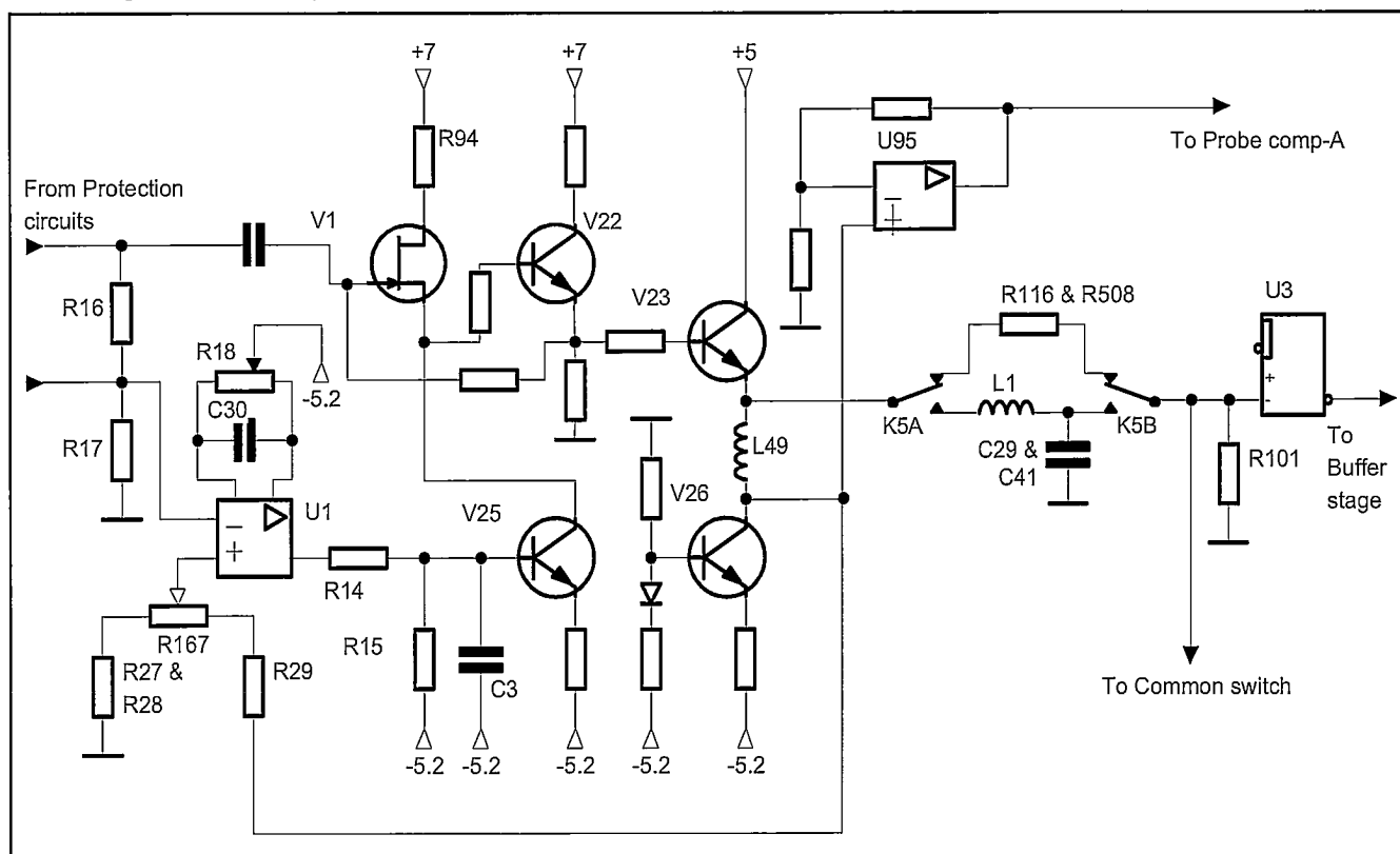
Figure 4-6 Impedance converter.
