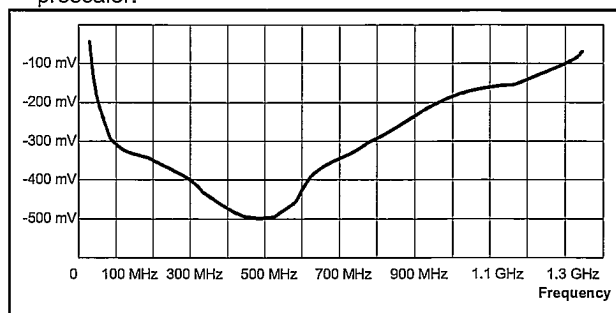
Figure 5-25 Typical Frequency Curve PM9621.
