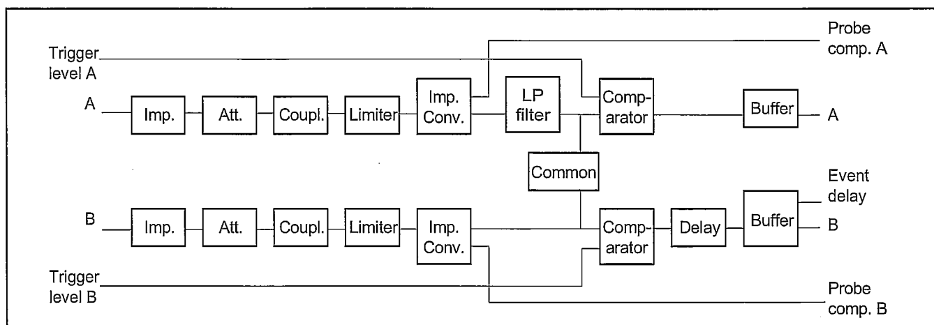
Figure 4-4 Input amplifier block diagram.
