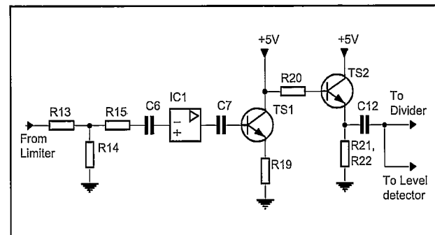
Figure 4-28 Amplifier circuits.
