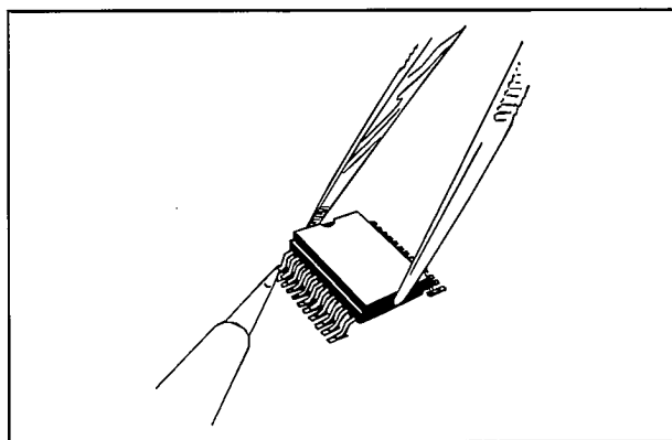
Figure 9-4 Attach the IC to the pad with solder.
