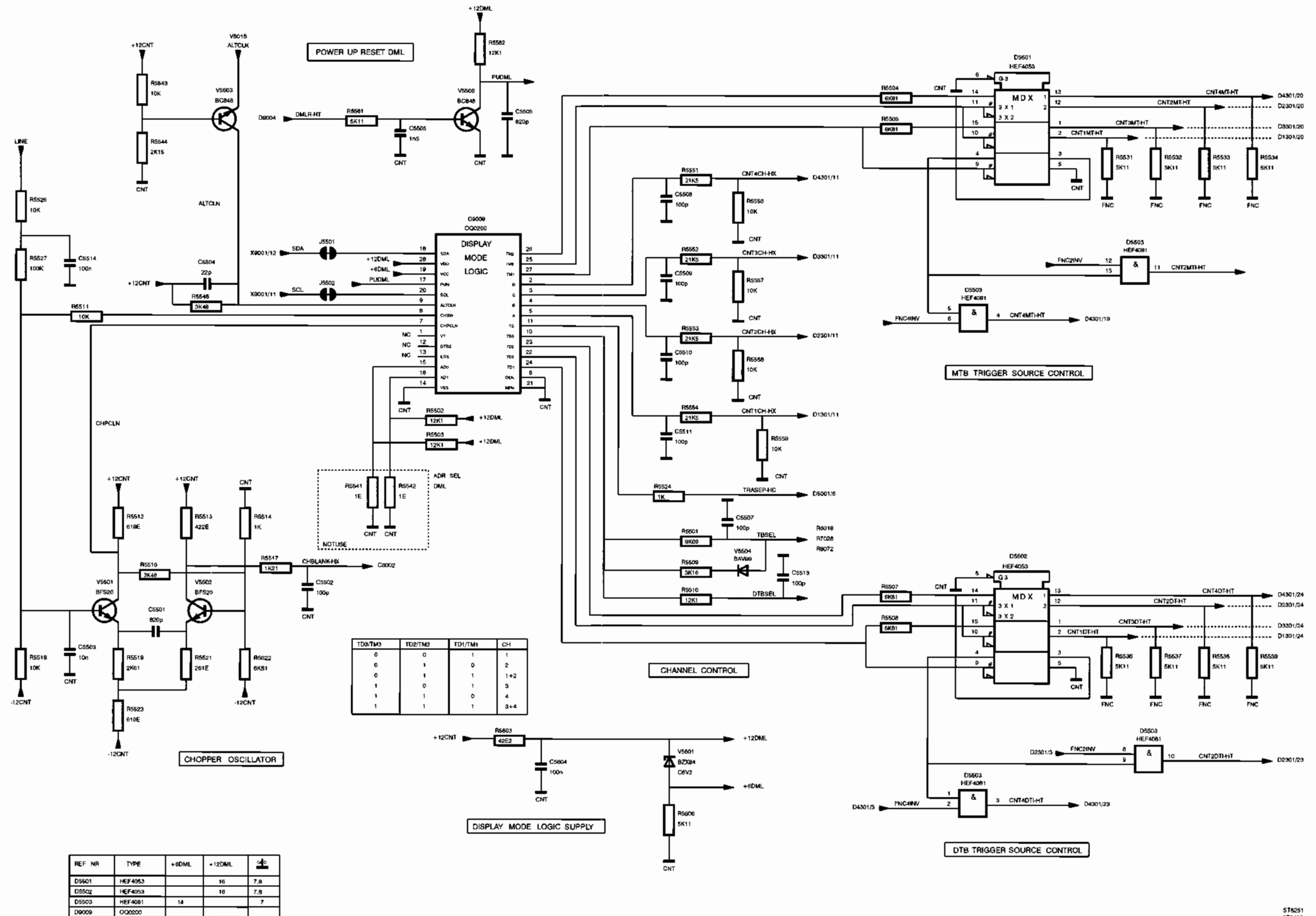
Diagram 10 - Display and trigger control
