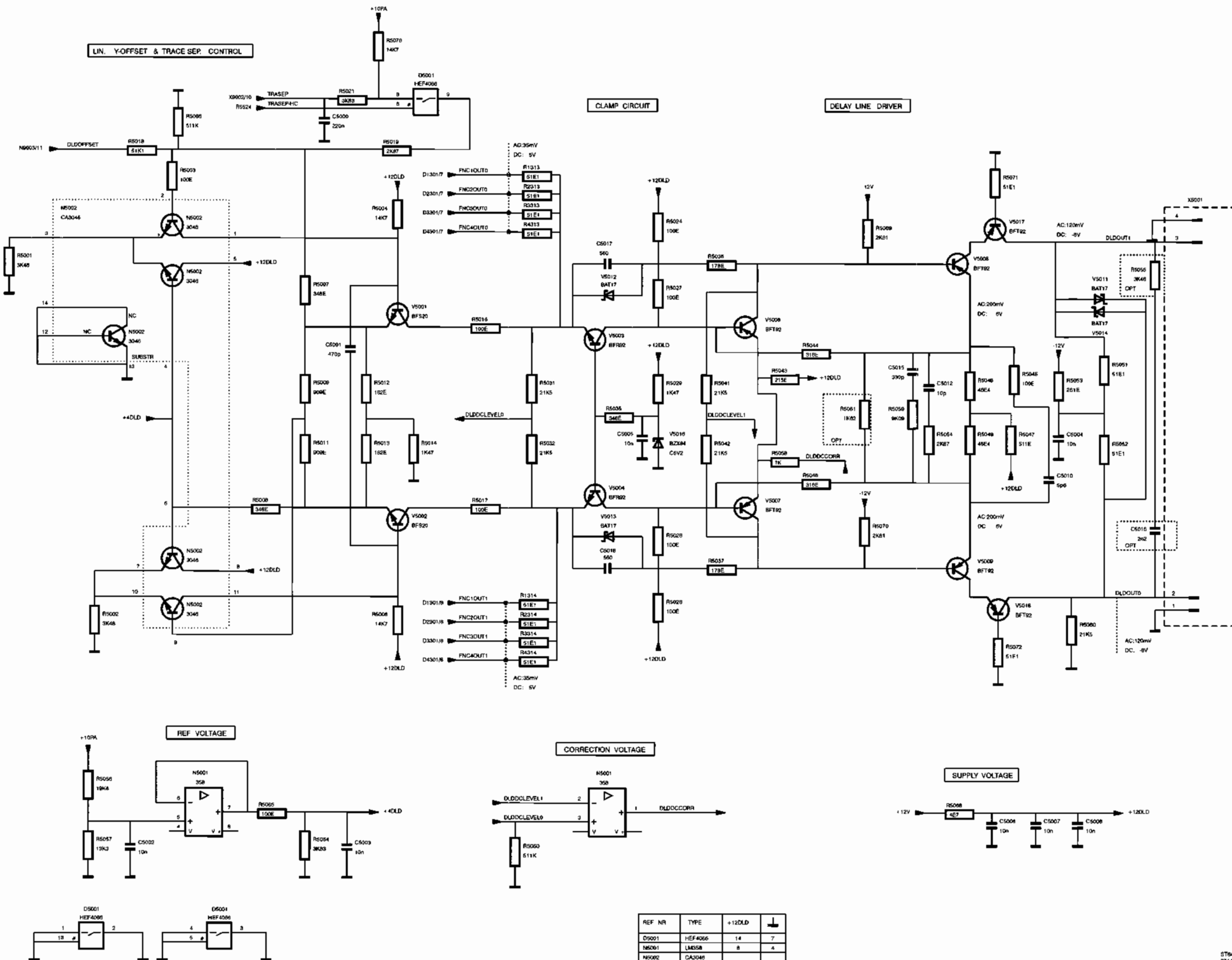
Diagram 9 - Delay line driver (PM3394A/92A/90A)
