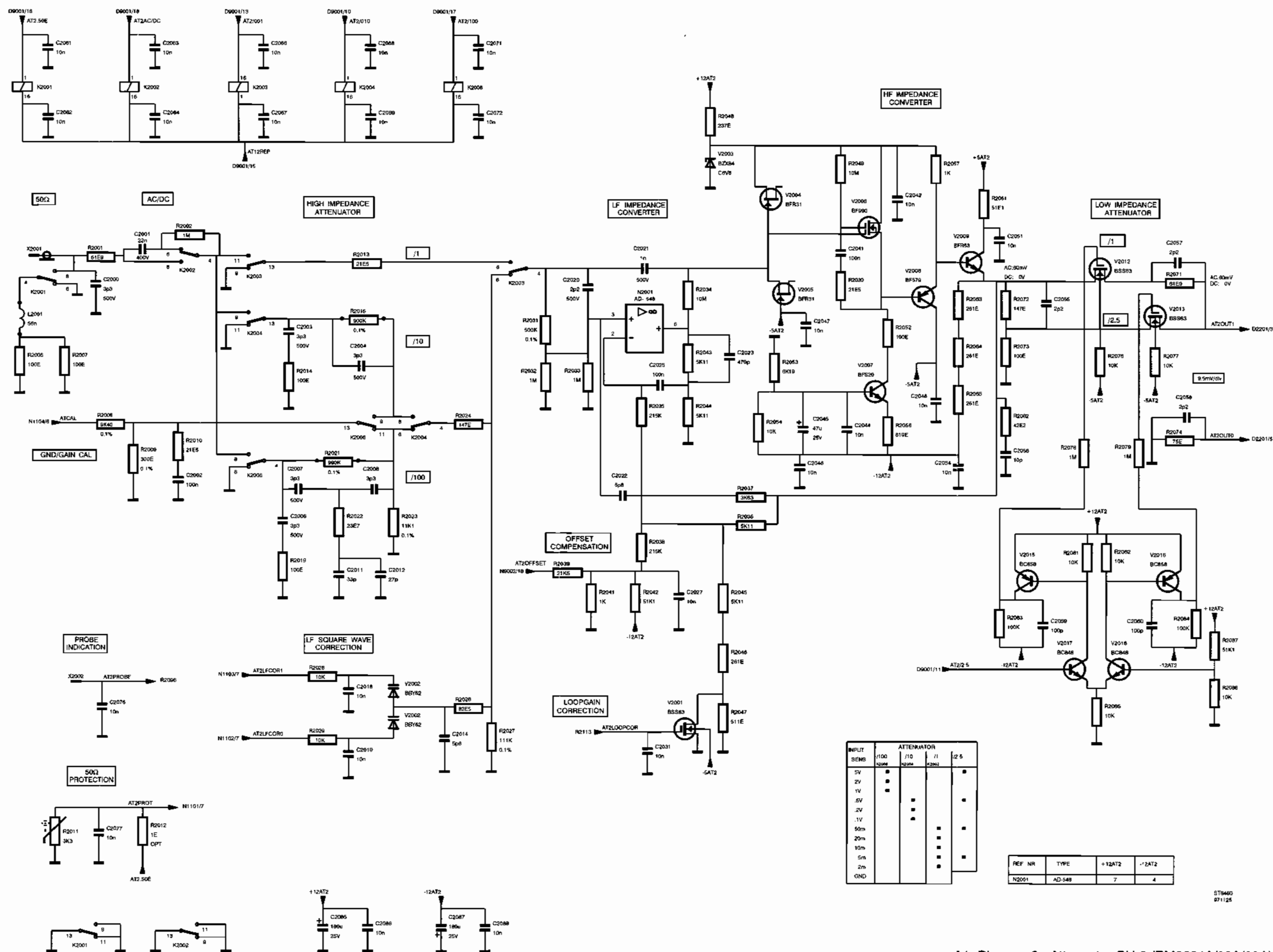
A1; Diagram 2 - Attenuator CH 2 (PM3394A/92A/90A)
