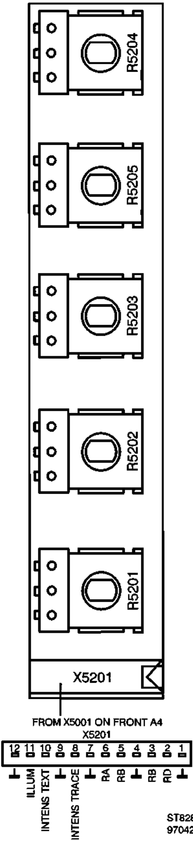
Lay-out 2; Large component side of CRT controls unit A5
