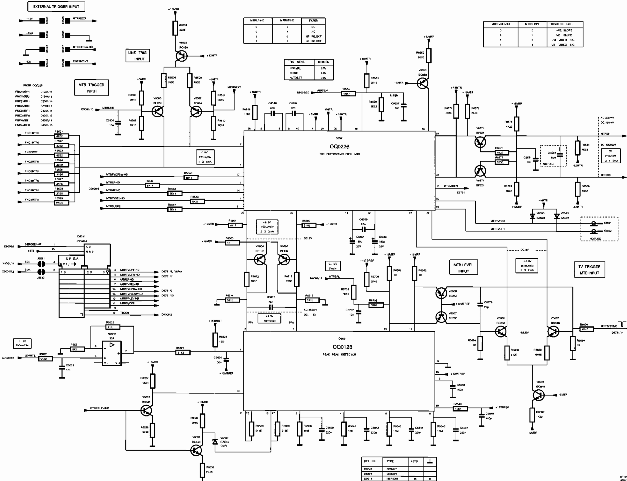
Diagram 12 - MTB trigger
