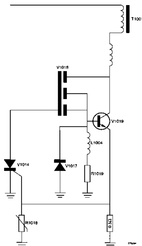
Figure 5.5 Converter circuit
