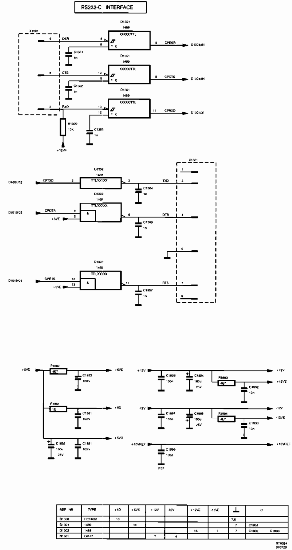
A3 - Diagram 3; Auxiliary circuits
