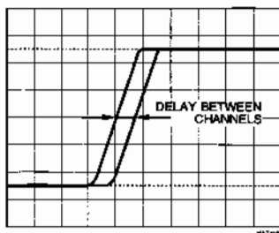
Figure 6.3 Delay difference \leq 0.13 div in PM3390A/92A/94A or \leq 0.05 div in PM3370A/80A/82A/84A.
