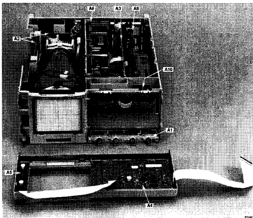
Figure 4.1 Unit Locations
