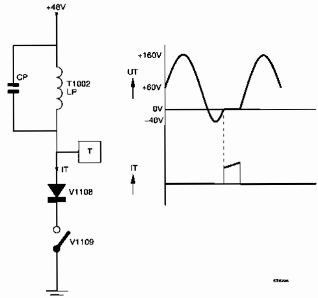
Figure 5.7 High tension generator
