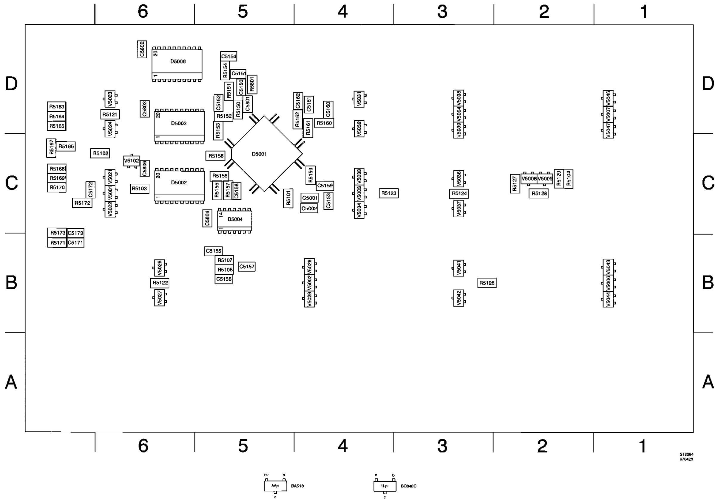
Lay-out 2 - Small component side of front unit A4
