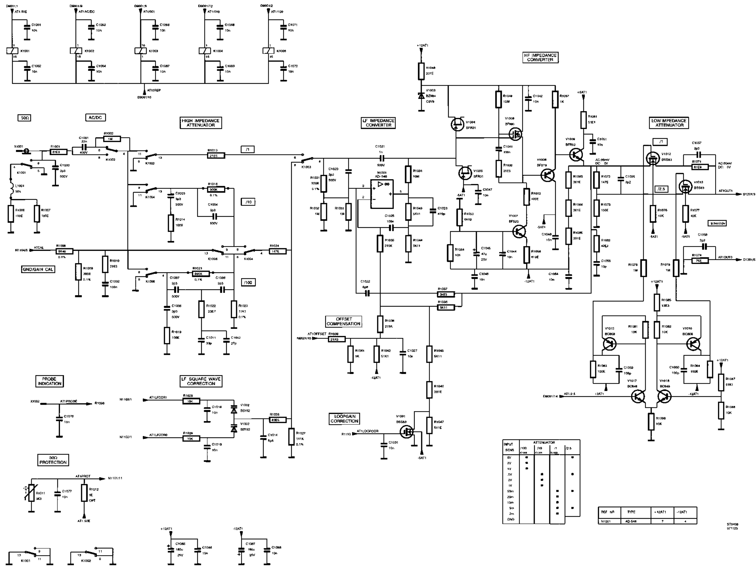
A1; Diagram 1 - Attenuator CH 1 (PM3394A/92A/90A)
