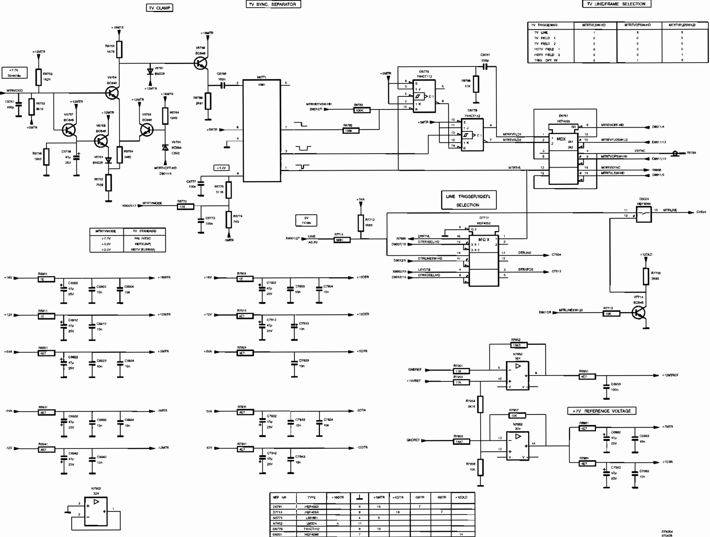
Diagram 13 - TV/line trigger
