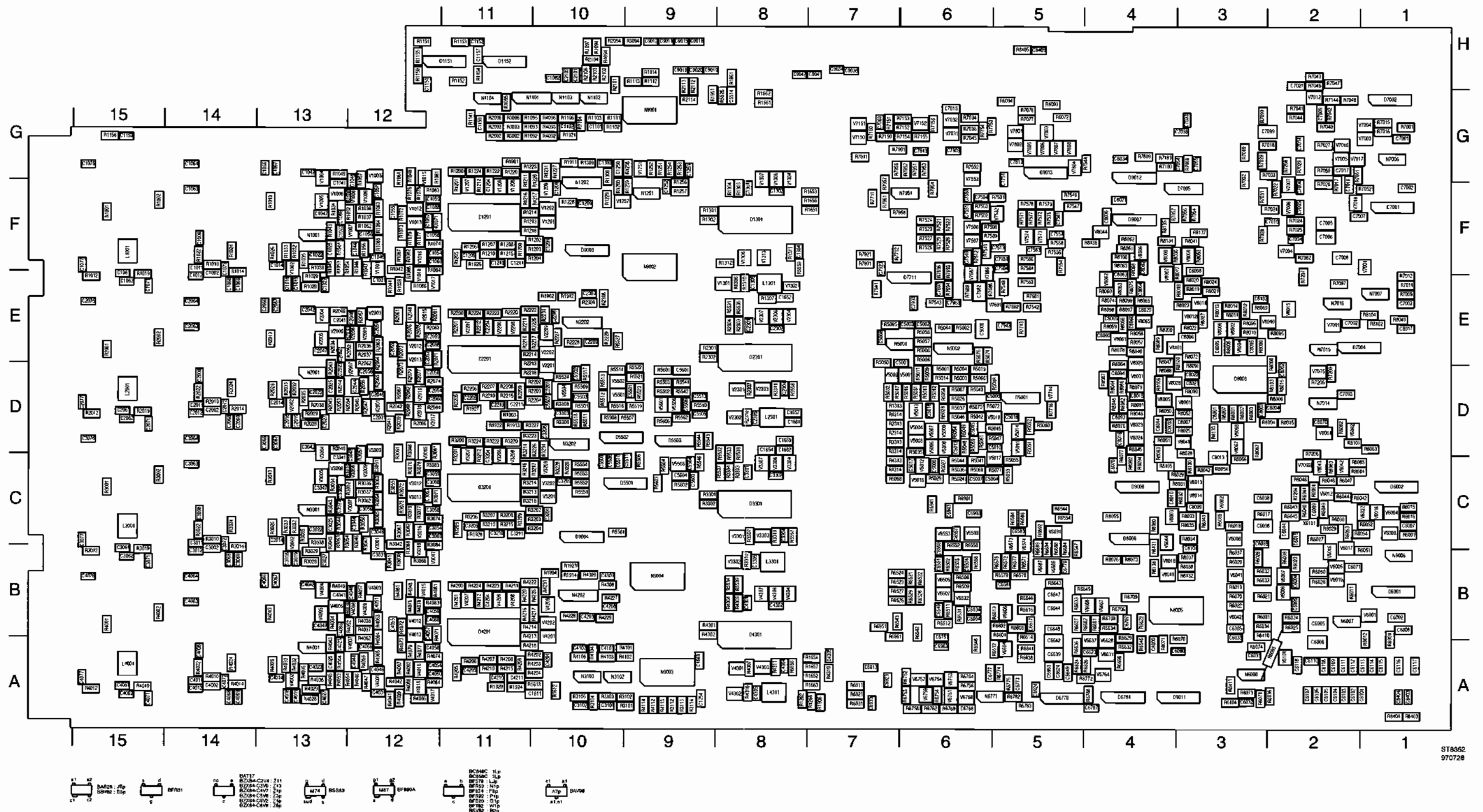
Lay-out 2 - Small component side of signal unit A1
