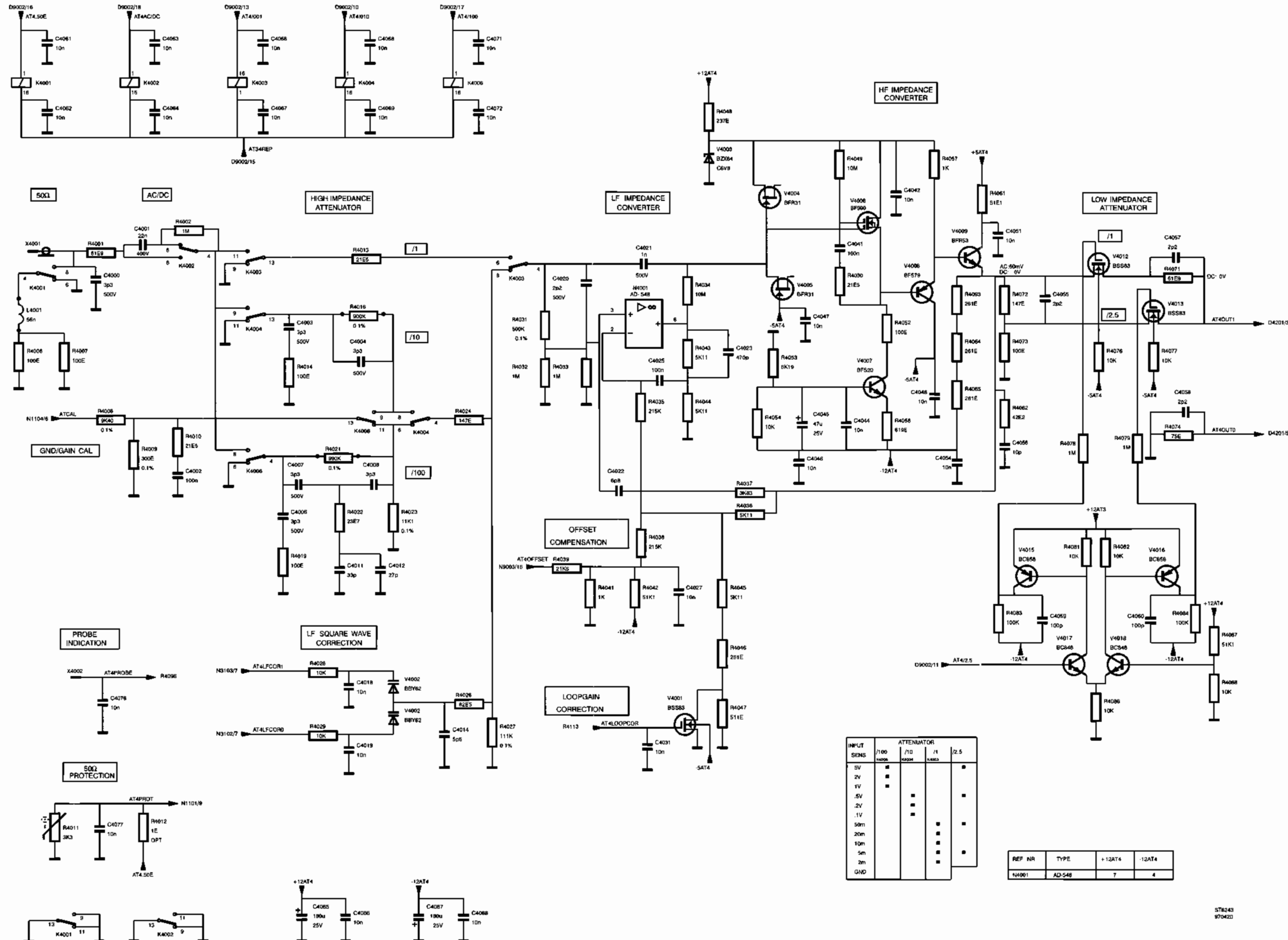
Diagram 4 - Attenuator CH 4 (PM3394A)
