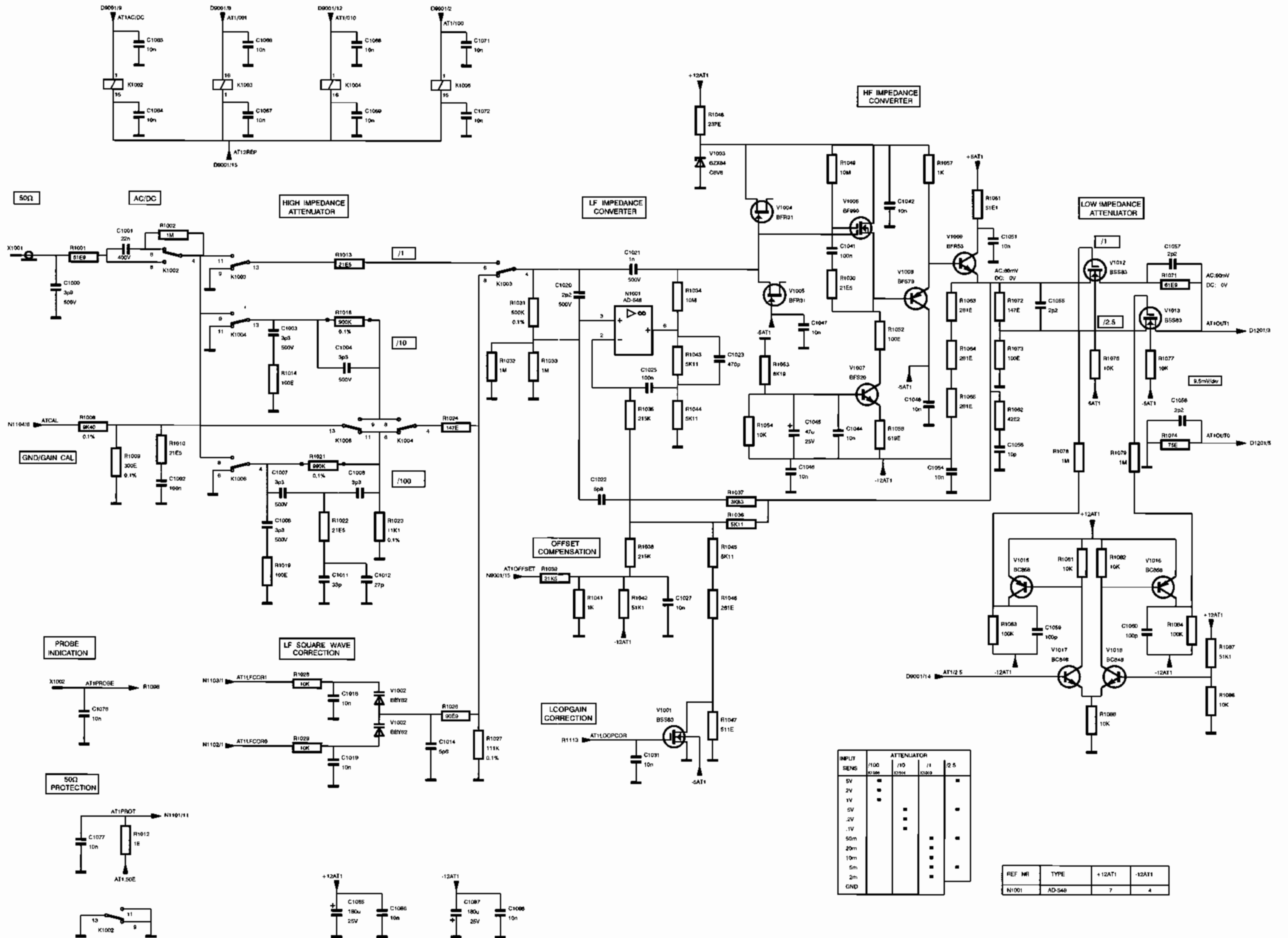
A1; Diagram 1a - Attenuator CH 1 (PM3384A/80A/70A)
