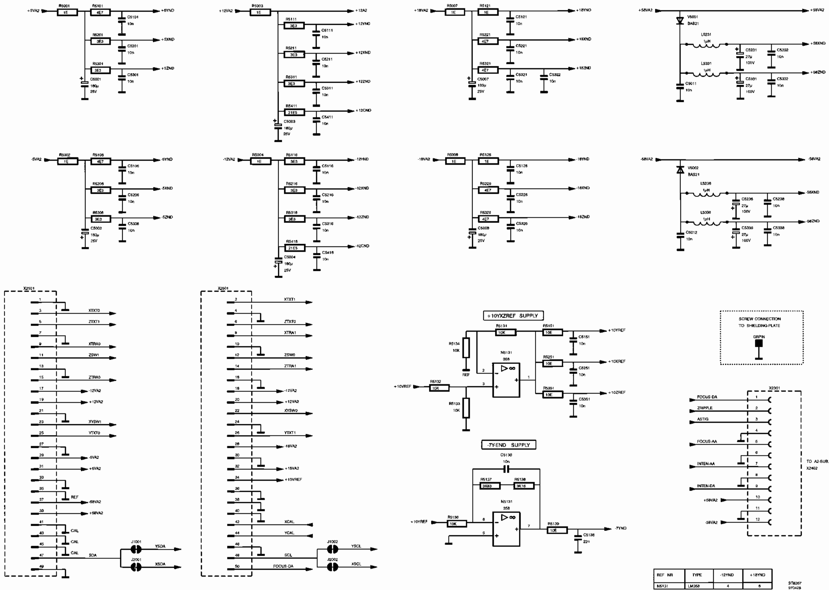
A2 (200 MHz) - Diagram 6 ; Supply circuits
