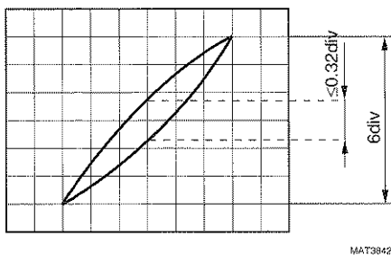
Figure 4.6 Phase shift between horizontal and vertical channel
