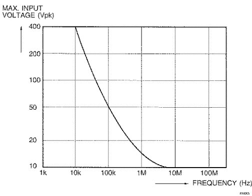
Figure 1.1 Max. input voltage versus frequency
