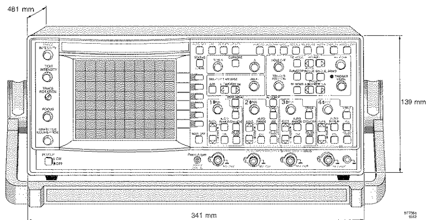
Figure 1.1 Dimensions
