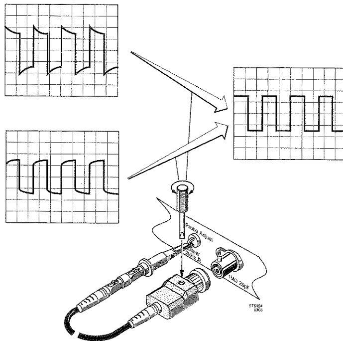
Figure 3.1 Probe adjustment
