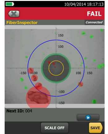
FiberInspector probe
