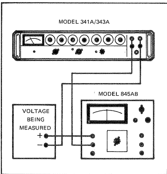
Figure 2-3. DIFFERENTIAL VOLTMETER
