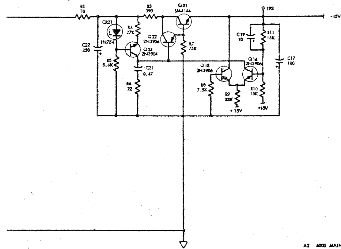
-15 VOLT AUXILIARY SUPPLY
