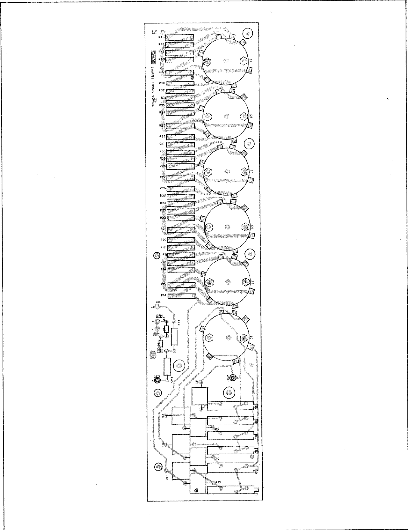
Figure 5-12. SAMPLE STRING P/C ASSEMBLY (343A)
