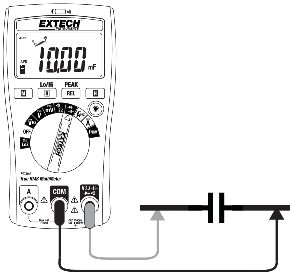
Fig 4-7 CAPACITANCE MEASUREMENTS
