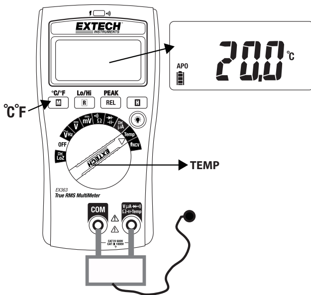
Fig 4-9 TEMPERATURE MEASUREMENTS
