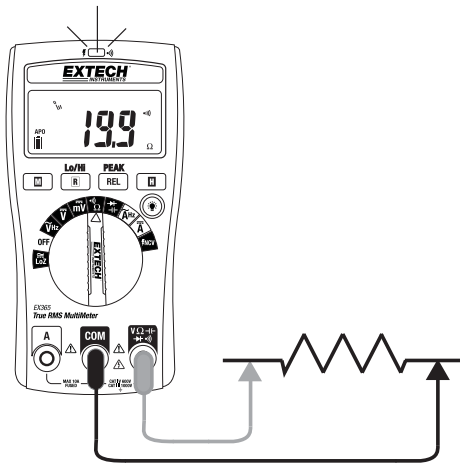
Fig 4-6 RESISTANCE/CONTINUITY MEASUREMENTS
