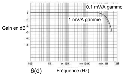
Figure 6(a – d): Courbe Gain/Fréquence @ 1 A crete, typique
