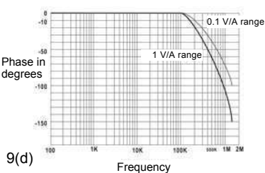
Figure 9(a - d): Phase versus Frequency @ 1 A peak, typical
