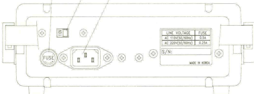
Fig 2-2. REAR PANEL
