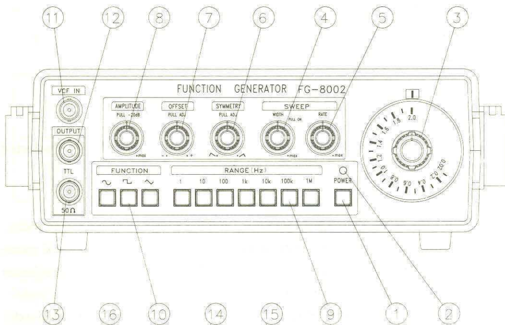
Fig 2-1. FRONT PANEL
