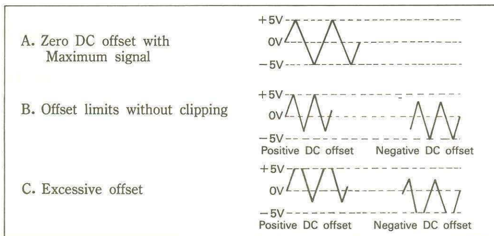
Fig 2-4. DC offset control
