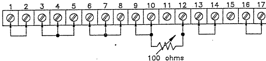
Figure 4. Remote programming by External Resistance, Current Mode
