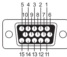
Schematic
