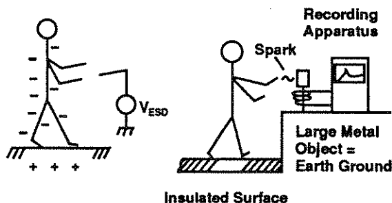
FIGURE 1: How human ESD models are derived: First, the open circuit voltage on the fingertip is measured. Then the short circuit current is monitored during discharge to ground.
