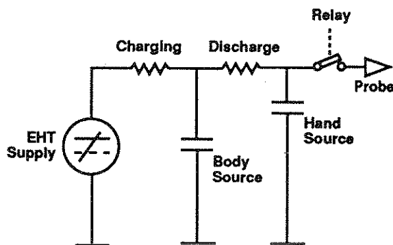
FIGURE 3 ESD simulator circuit. Earlier simulators do not include the additional "hand" capacitance. The total capacitance is generally 150 pf, and the discharge resistance is 150 or 330 ohms, depending on the applicable standard.
