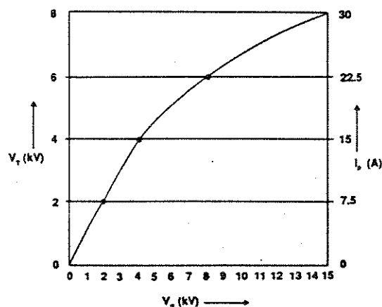
FIGURE 5: The peak current (IP) produced by through-air ESD simulators differs from the peak current produced by current injection techniques for the same applied voltage. The peak current produced by current injection techniques is proportional to the voltage of the simulator's capacitance (VT). However, the voltage for ESD simulator employing through-air discharge techniques is nonlinearly related to current. Corona effects which start to exhibit themselves above 4 kilovolts are one possible cause. VT is the voltage on the probe tip prior to discharge for a direct injection probe. VE is the voltage on the probe tip prior to discharge for a through-air type probe.
