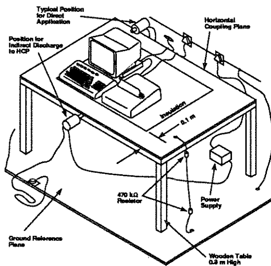
FIGURE 8: Table top units are tested atop a horizontal coupling plane (HCP). The HCP is resistively grounded to the ground reference plane.
