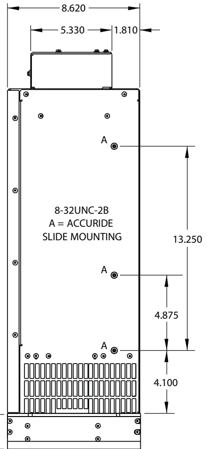
Side View
