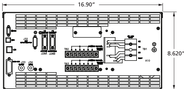
Rear View
