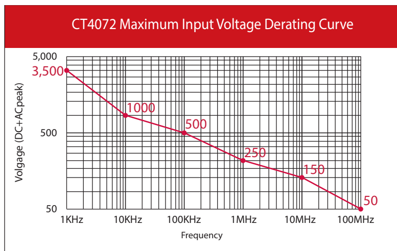
Figure 3 CT4072: Derating Curve
