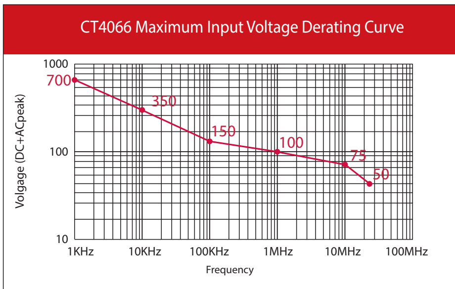
Figure 2 CT4066: Derating Curve
