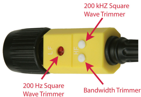
Figure 2: Frequency Compensation Trimmer
