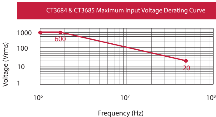
Figure 3 Derating Curve
