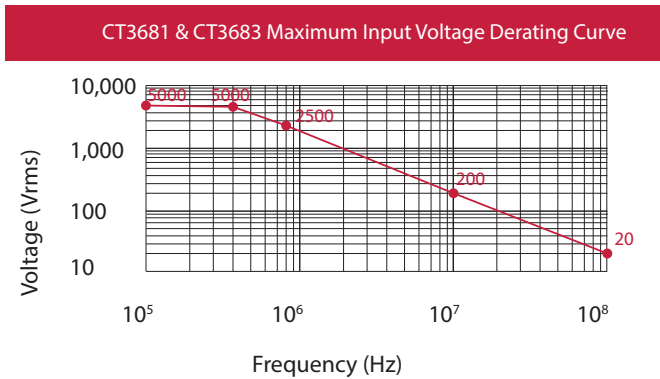
Figure 3 Derating Curve
