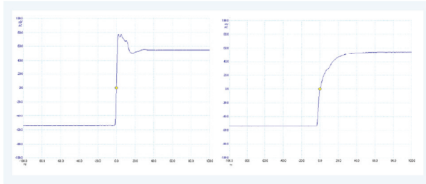
Figure 2: Over/Under Compensation
