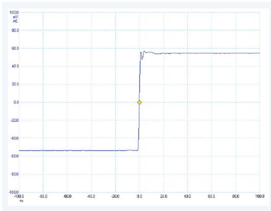
Figure 3: Good Compensation
