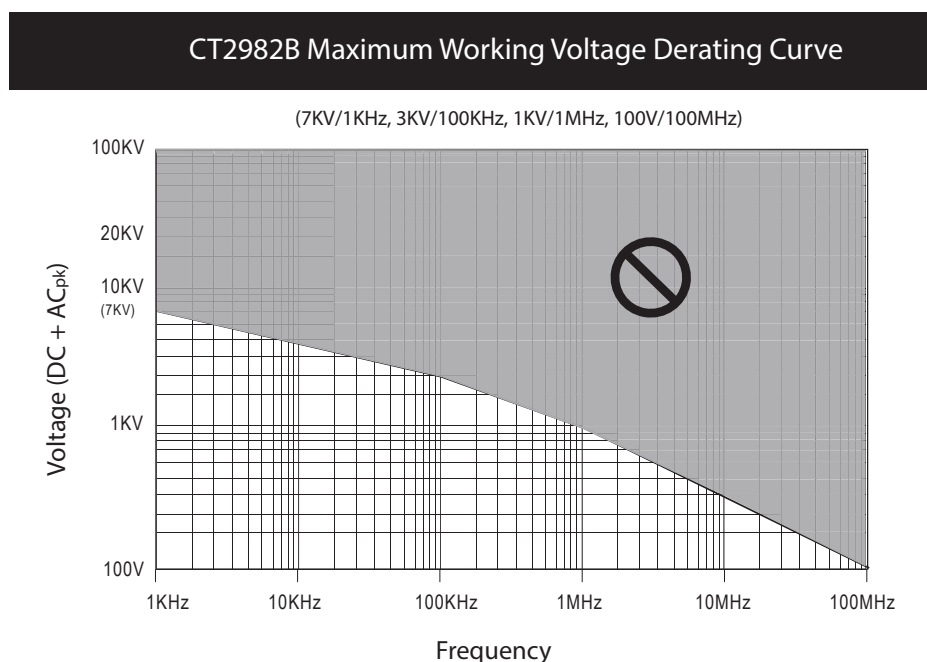
Figure 4: Voltage Derating Curve
