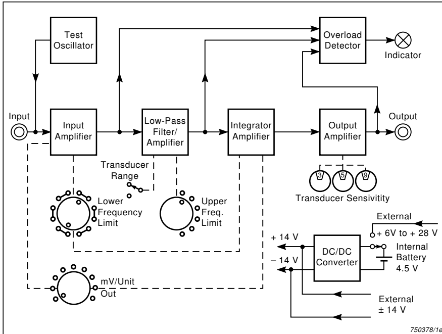
Fig. 1 Block diagram of Type 2635
