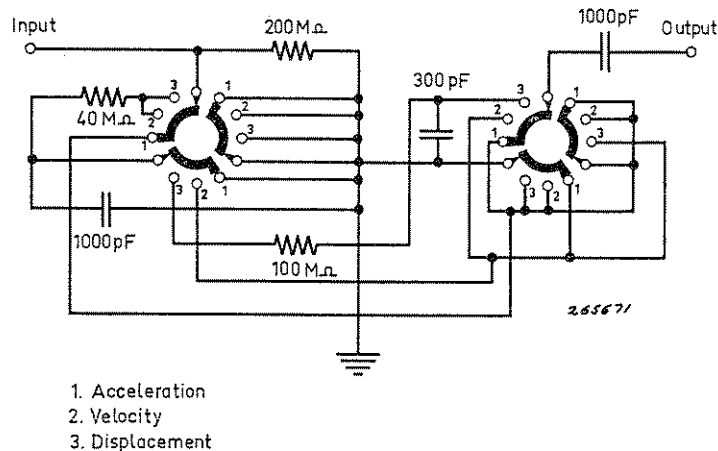
Fig. 4.3. Circuit diagram for the Integrator ZR 0020.
