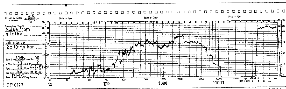
Fig. 9.10. Spectrogram of the noise produced by a lathe.
