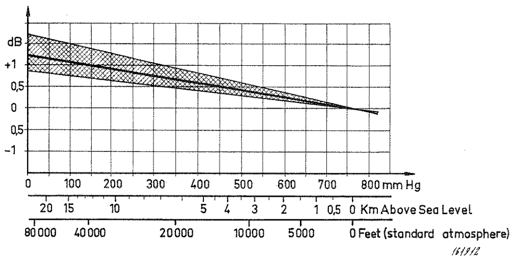
Fig. 5.2. Microphone sensitivity at 400 Hz (c/s) as a function of the static ambient pressure. The corresponding altitudes are also given on the curve.
