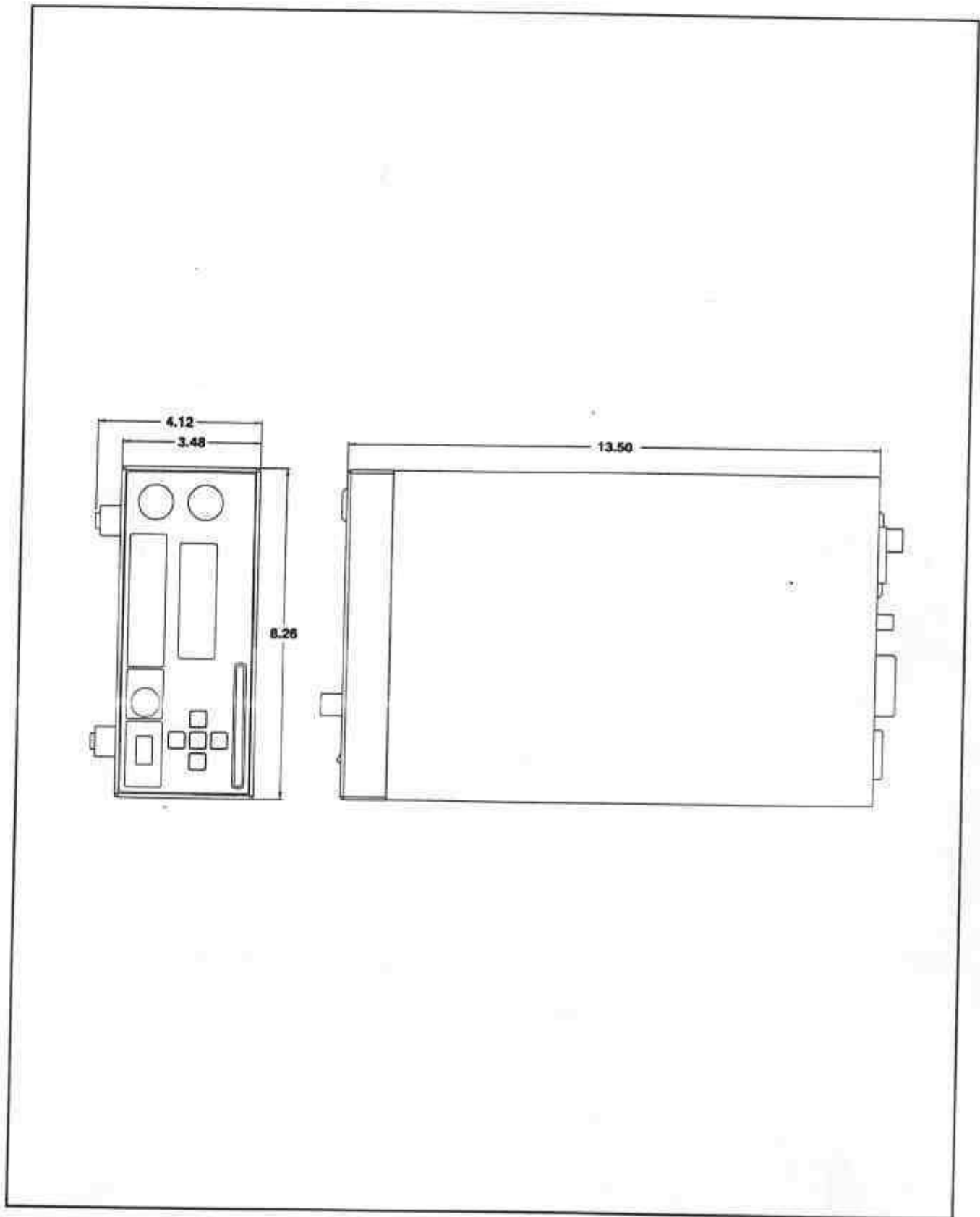
Figure 1-3. Outline Dimensions
