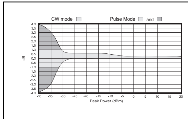
Temperature Influence ( \pm 4° from calibration)
