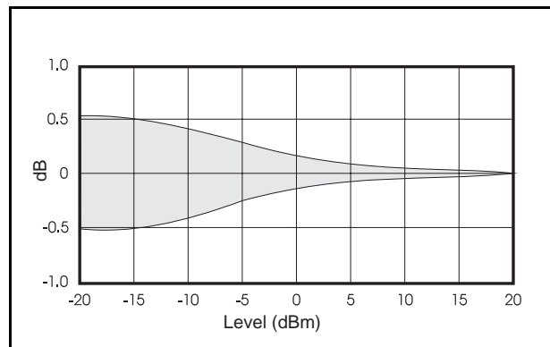
Temperature Influence ( \pm 4° from calibration)
