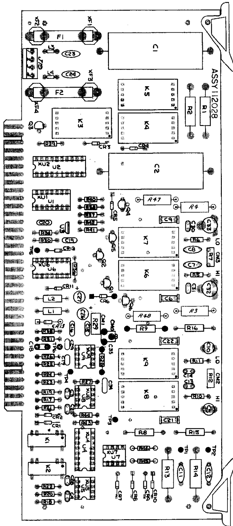
Figure 6-3. PWA '1121' Input (A0)
