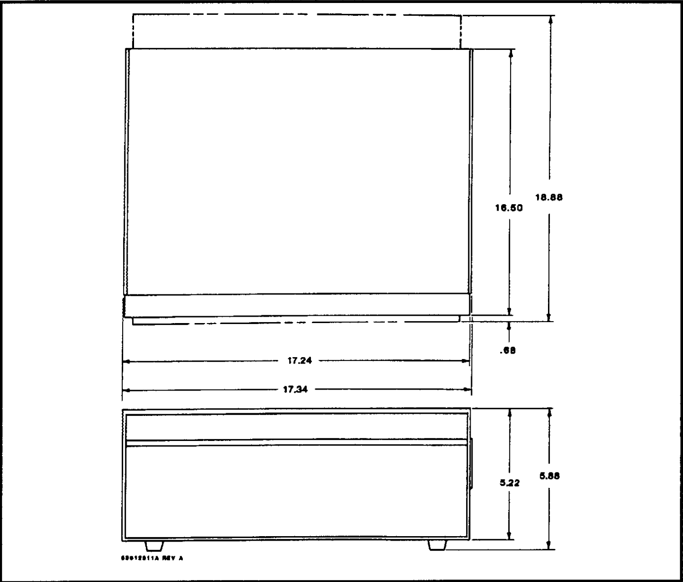
Figure 1-1. Outline Dimensions.
