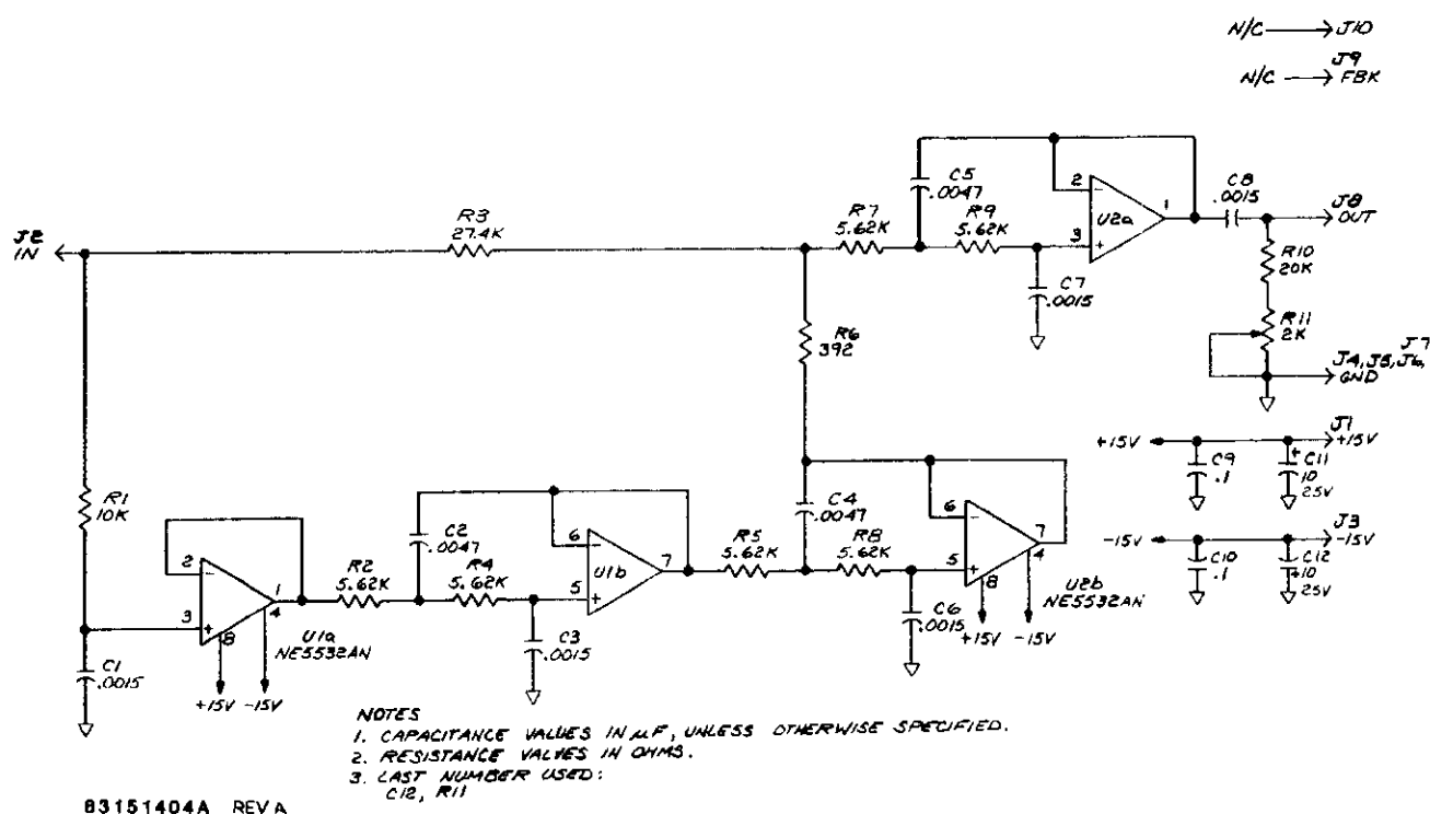
Figure 7-37. CCIR Board A1A32,A33 Schematic.
