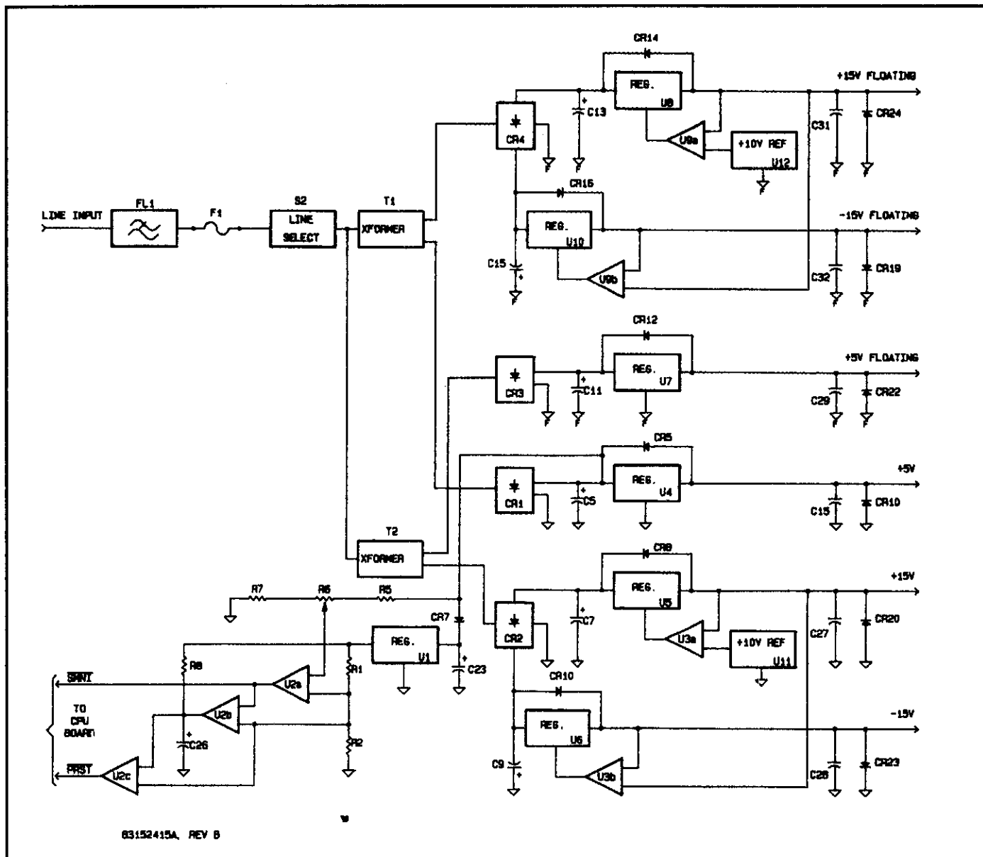
Figure 4-2. Power Supply Circuits Block Diagram.
