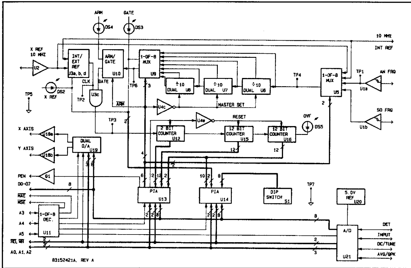
Figure 4-4. Frequency Counter Circuits Block Diagram
