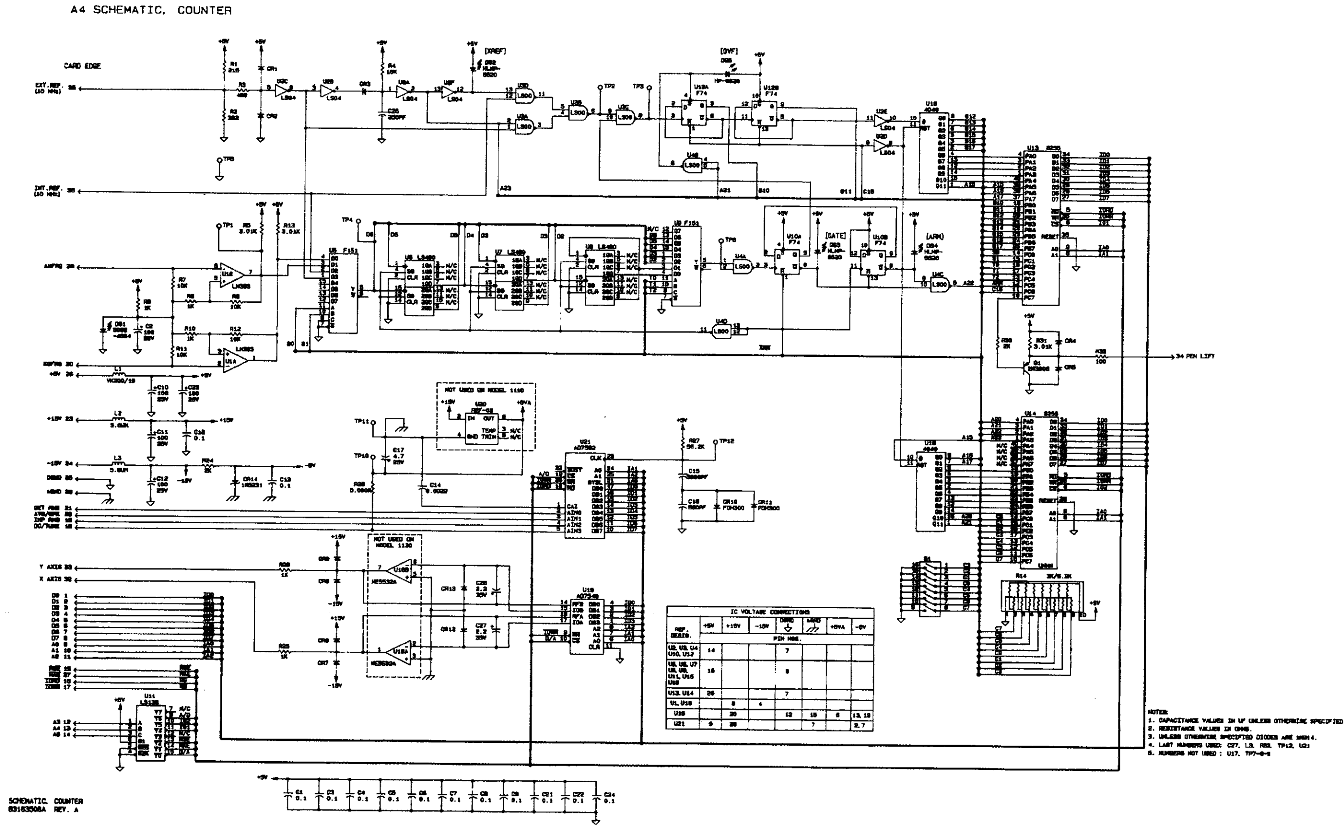
Figure 7-13. Counter Board A4 Schematic.
