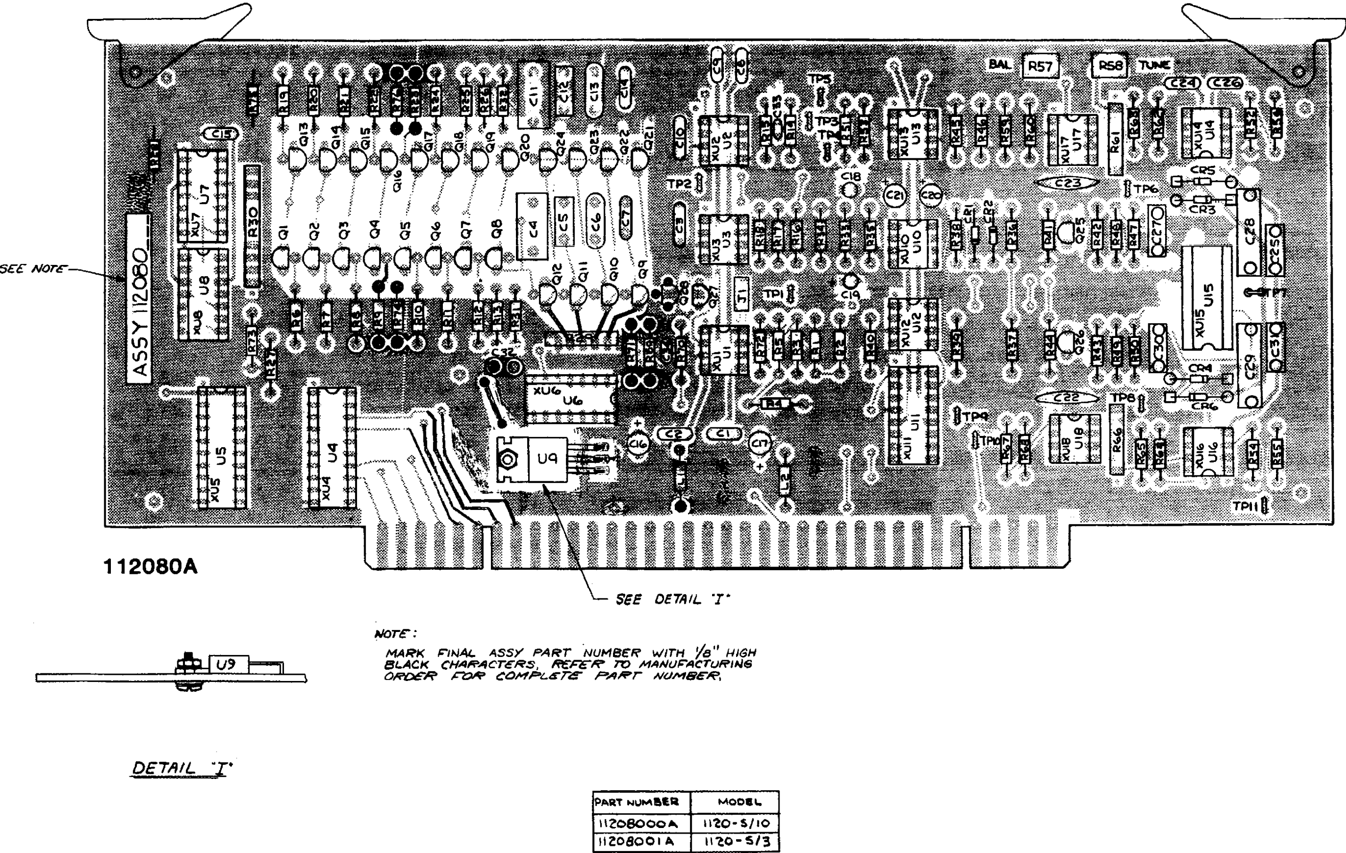
Figure 7-6. Notch Board A2 Parts Location Diagram.
