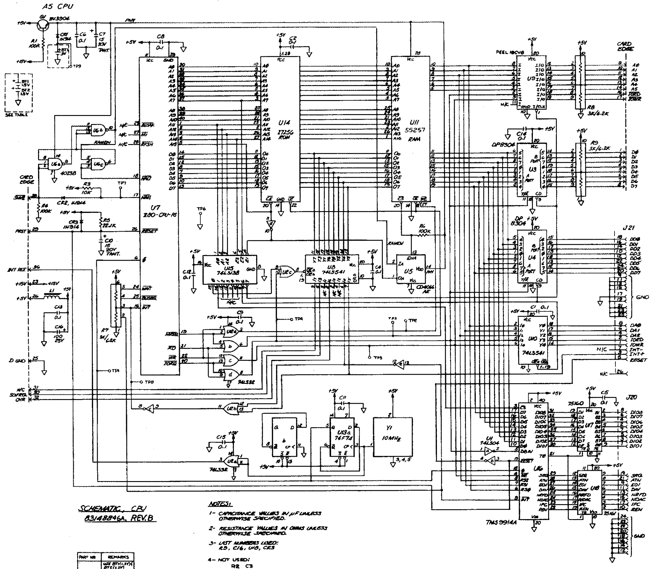
Figure 7-15. C.P.U. Board A5 Schematic.
