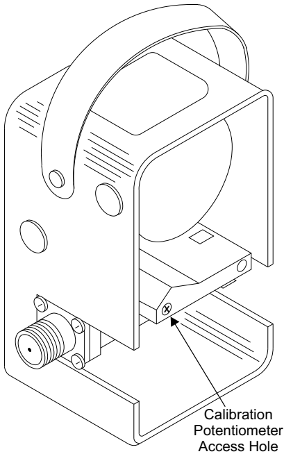
Figure 10 Calibration Potentiometer
