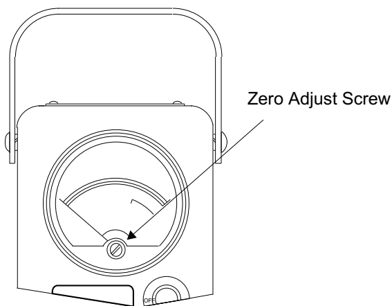
Figure 6 Zero Adjustment
