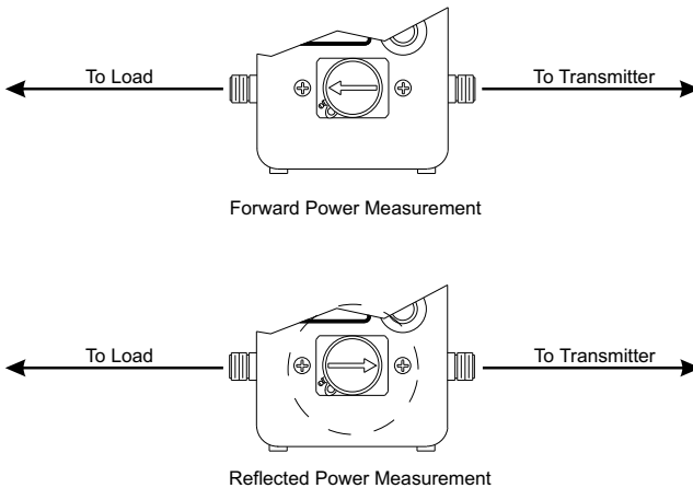
Figure 5 Measurement Direction
