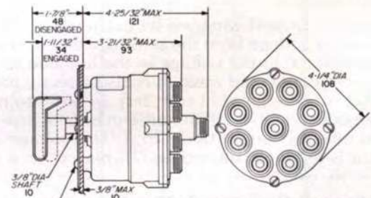
MOUNTING DIMENSIONS 7/32" (6mm) MTG HOLES FOR FOUR 10-32 SCREWS SPACED AT 90° ON 1 1/4" (33mm) RADIUS
