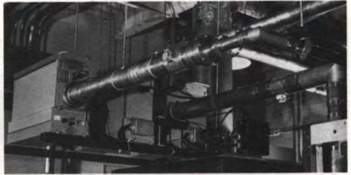
This TT50FL dual transmitter installation at WKYC-TV is the first in the country. Shown above are three TERMALINE "Reject Loads" with their THRULINE Wattmeters. The 50kW Test Load/Wattmeter is switched remotely (including water flow) from the studio 10 miles distant, where the reject power levels and main feed power are monitored (below left and right).
