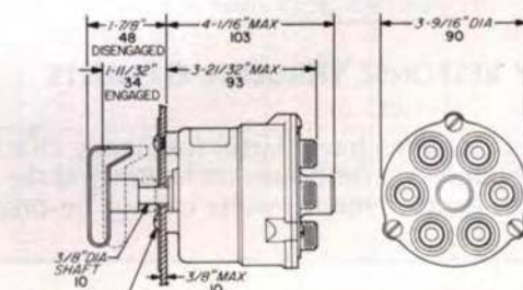
MOUNTING DIMENSIONS 7/32" (6mm) MTG HOLES FOR THREE 10-32 SCREWS SPACED AT 120° ON 1 1/4" (32mm) RADIUS
