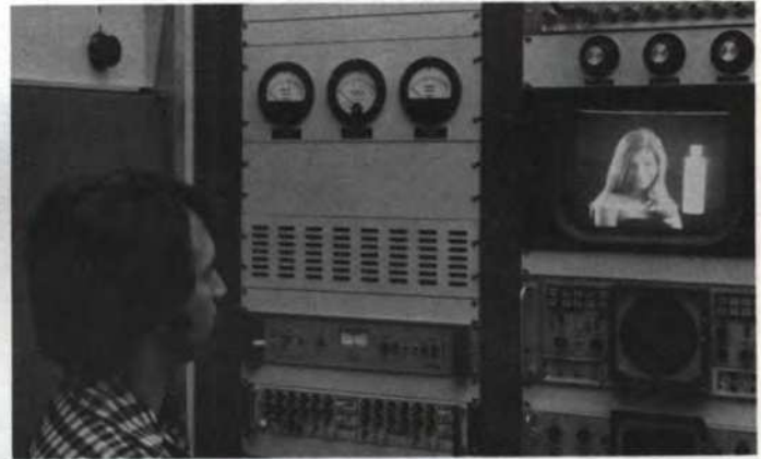
This TT50FL dual transmitter installation at WKYC-TV is the first in the country. Shown above are three TERMALINE "Reject Loads" with their THRULINE Wattmeters. The 50kW Test Load/Wattmeter is switched remotely (including water flow) from the studio 10 miles distant, where the reject power levels and main feed power are monitored (below left and right).
