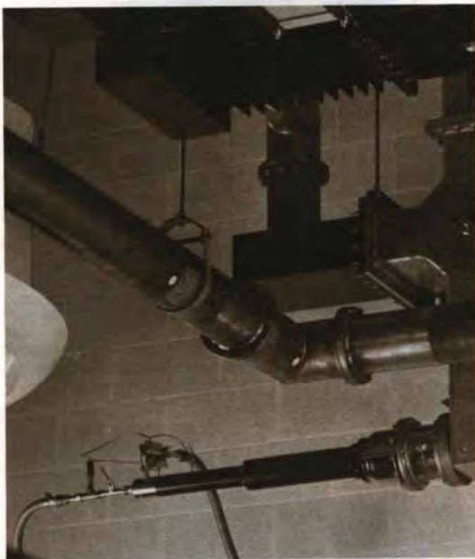
During measurement and maintenance, station WCLQ-TV channel 61 dissipates visual and aural power in this 80kW Econoload® model 8790 mounted overhead on the waveguide switch following the filterplexer.
