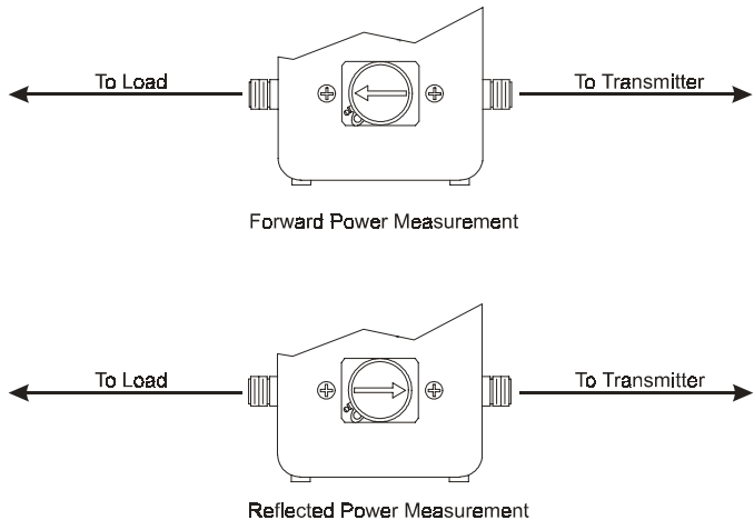
Figure 7 Element Direction
