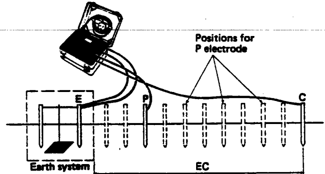
Figure 4 Instrument connection for slope method
