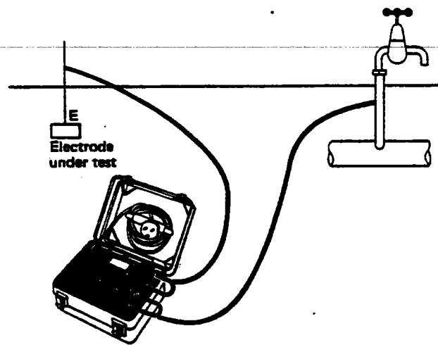
Figure 5 Connection to a water main
