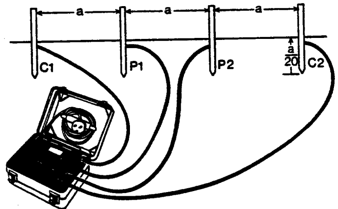
Figure 7 Connections for resistivity tests
